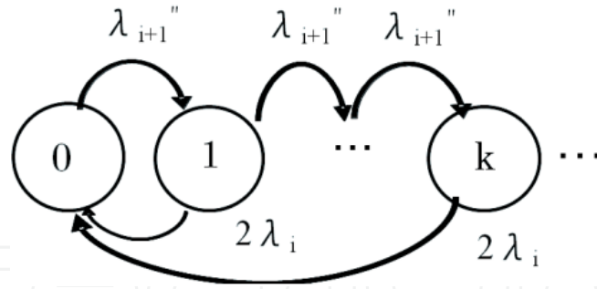
Figure 4. State transition rate diagrams of full aggregation
