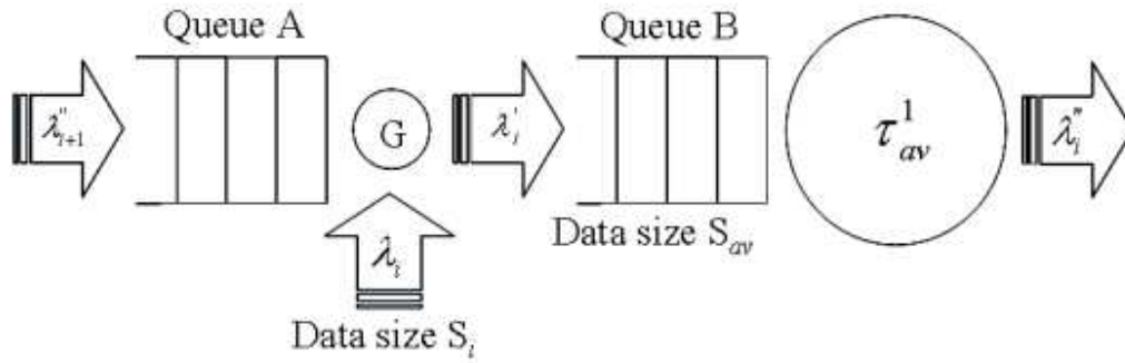
Figure 3. Analytical model of full aggregation
