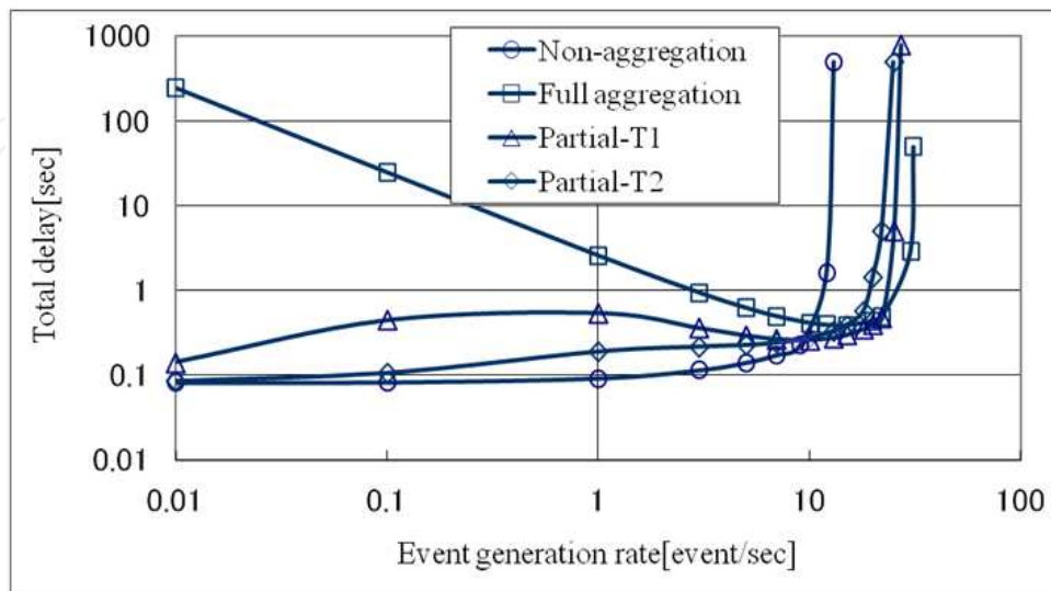
Figure 7. Total delay
