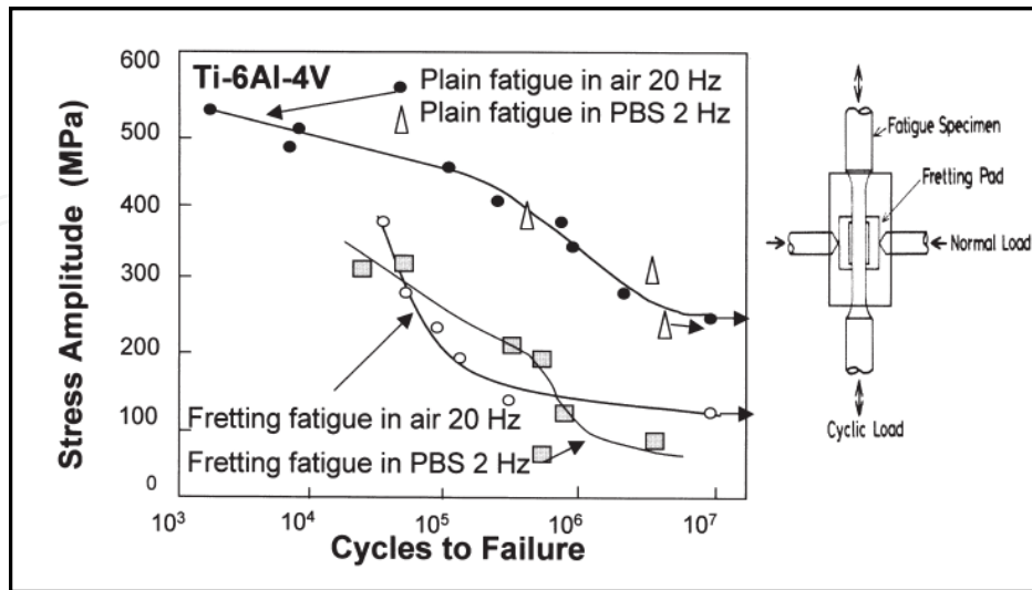
Figure 5. Fretting fatigue in PBS environment of Ti-6Al-4V [12]
