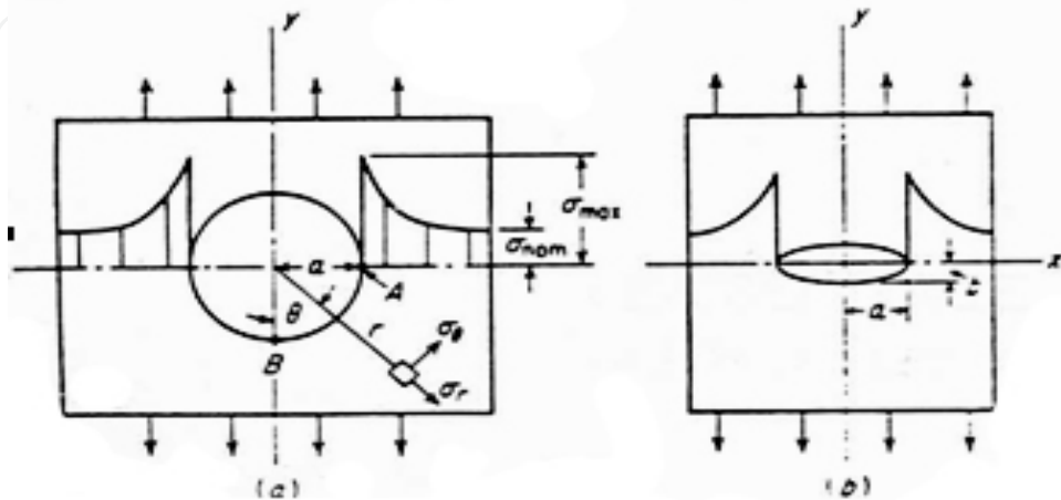
Figure 8. Schematic of distribution around a crack perpendicular to applied stress [20]
