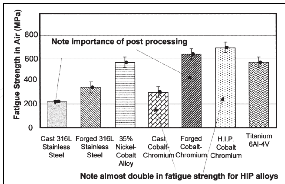
Figure 3. Fatigue strength of some common implant alloys [1]
