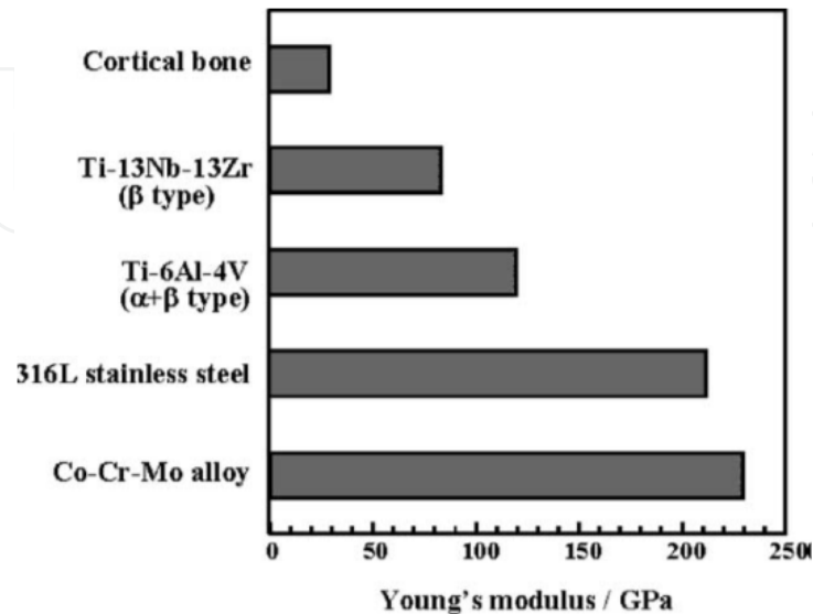
Figure 2. Comparison of Young's modulus of cortical bone, \beta type Ti-13Nb-13Zr, \alpha + \beta type Ti-6Al-4V, 316L stainless steel and Co-Cr-Mo alloy for biomedical applications [10]
