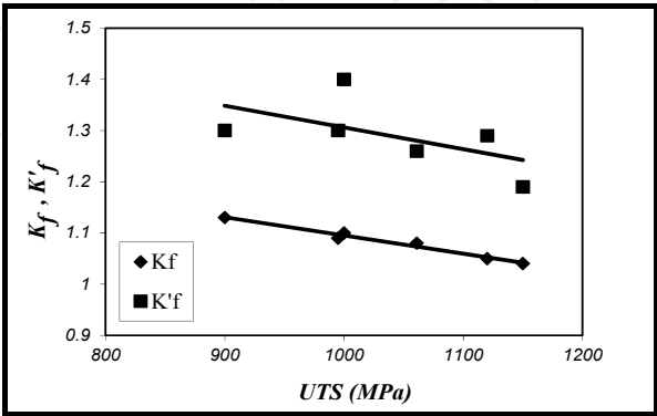
Figure 10. Effect of tensile strength on K_f and K'_f [4]
