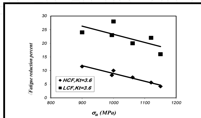
Figure 7. Effect of tensile strength on fatigue reduction in Ti-6Al-4V [4]
