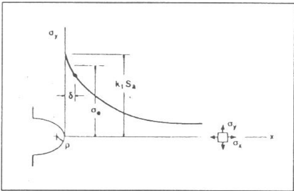
Figure 11. Interpretation of the fatigue limit as the average stress over a finite distance \delta ahead of the notch [19]
