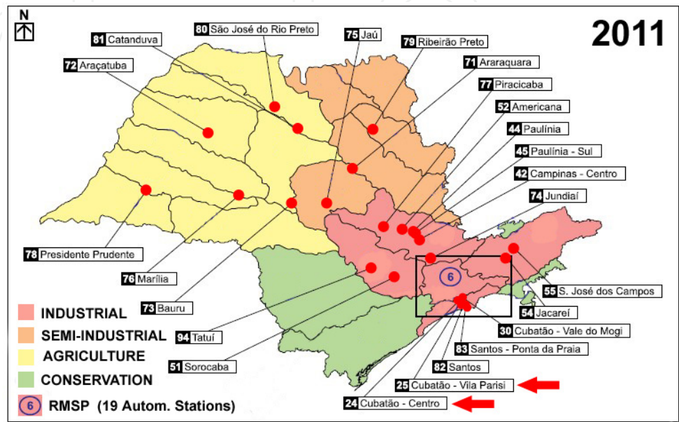
Figure 3. CETESB network of automatic monitoring stations in 2011. The shading indicates the principal land use in four schematic regions of the State, directly related to the type of emissions. Adapted from [9].
