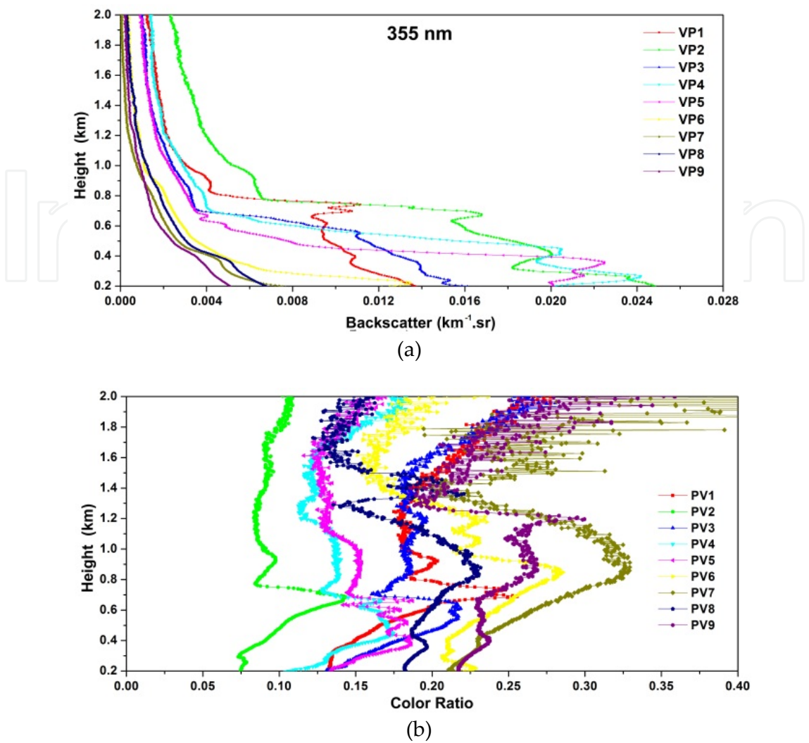
Figure 22. (a) Vertical profile of Backscatter Coefficient (BSC) at 355 nm; (b) Colour Ratio 532/355 nm. (After [33]).
