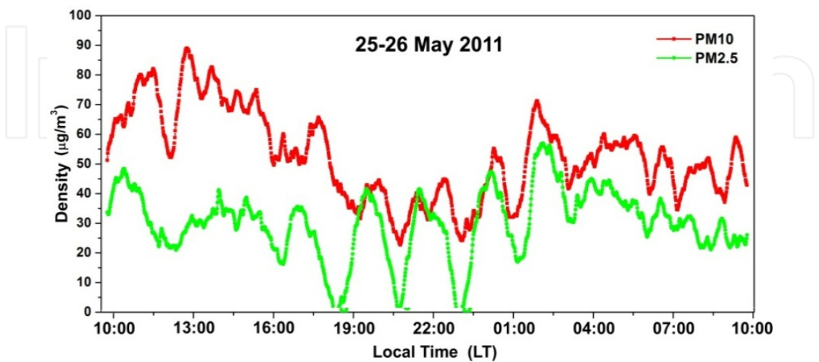
Figure 23. Concentrations of \text{PM}_{10} and \text{PM}_{2.5} from 10:00 LT on 25 May to 10:00 LT on 26 May 2011. (After [33]).
