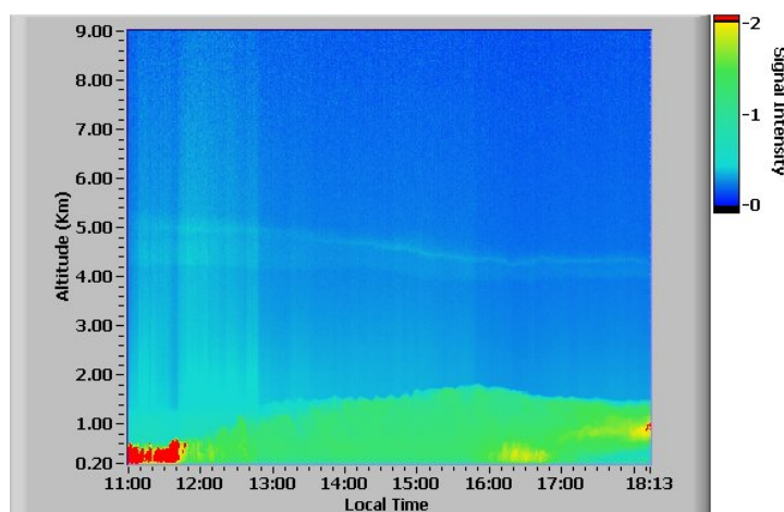
Figure 15. Lidar observations at IPEN in São Paulo, showing the range-corrected signal in arbitrary units, on 14 July 2008 between 11:00 and 18:13 LT. The plume identified in Figure 14 can be seen between 4-5 km AGL.
