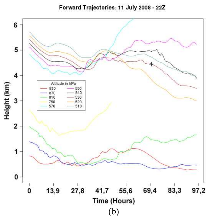
Figure 14. Forward trajectories initiated at different heights where a large fire was observed by IPMet's radars on 11 July 2008, 22:00 UT (19:00 LT). (a) The + indicates the position of the PPR and BRU radars; o indicates the position of the lidar in São Paulo (IPEN). (b) Forward trajectories plotted against height and time. The + indicates the position of IPEN, marking height and time of arrival matching exactly with the lidar observation (Figure 15).
