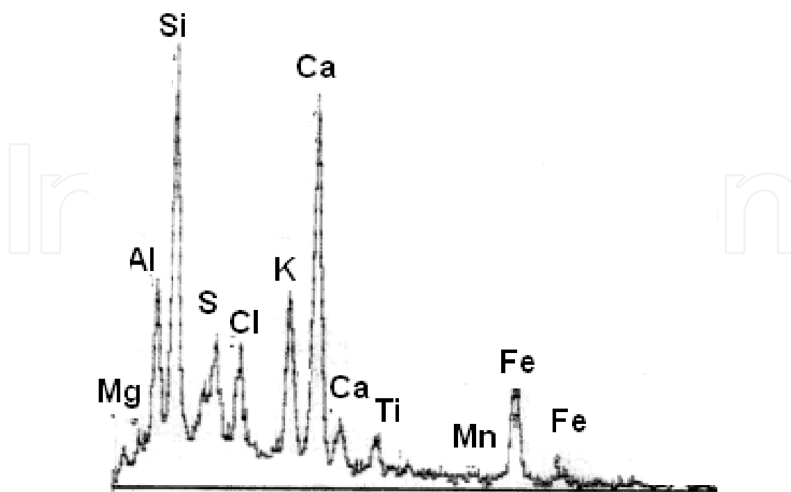
Figure 10. EDX spectrum of elemental chemical analysis of settled particulate matter
