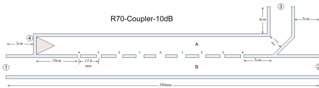
Figure 11. The R70 directional coupler, C = 10 dB by two rows of 9-elements
