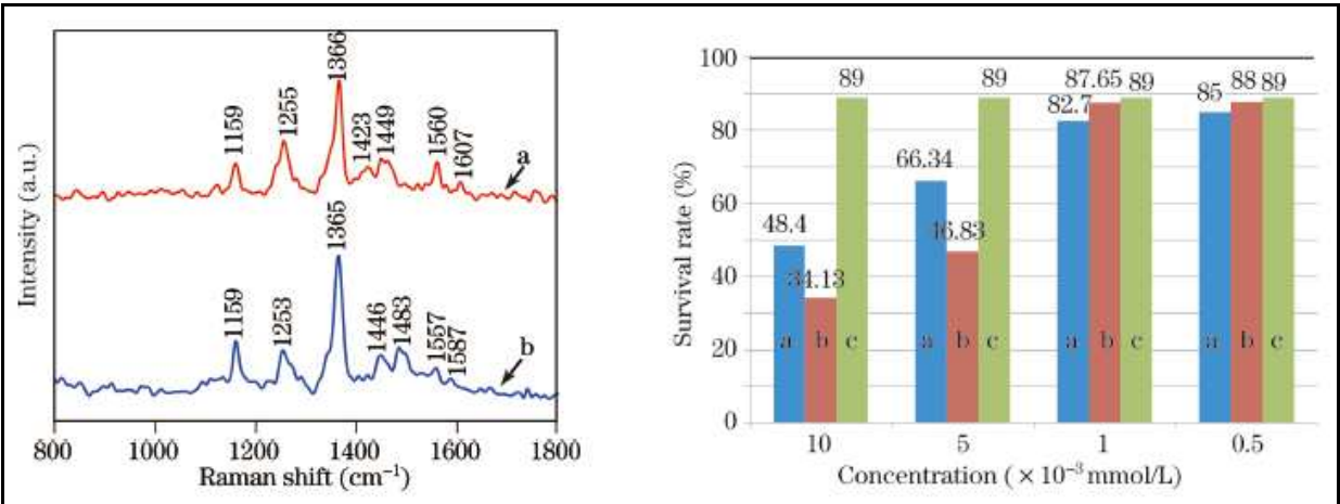
Fig. 5. Left side shows SERS spectra of drug in (a) solution and (b) living cells and right side shows viability of cells treated with different concentrations of drug and silver nanoparticles. (a) Pure drug; (b) Drug and silver nanoparticle complex; (c) pure silver nanoparticles.
