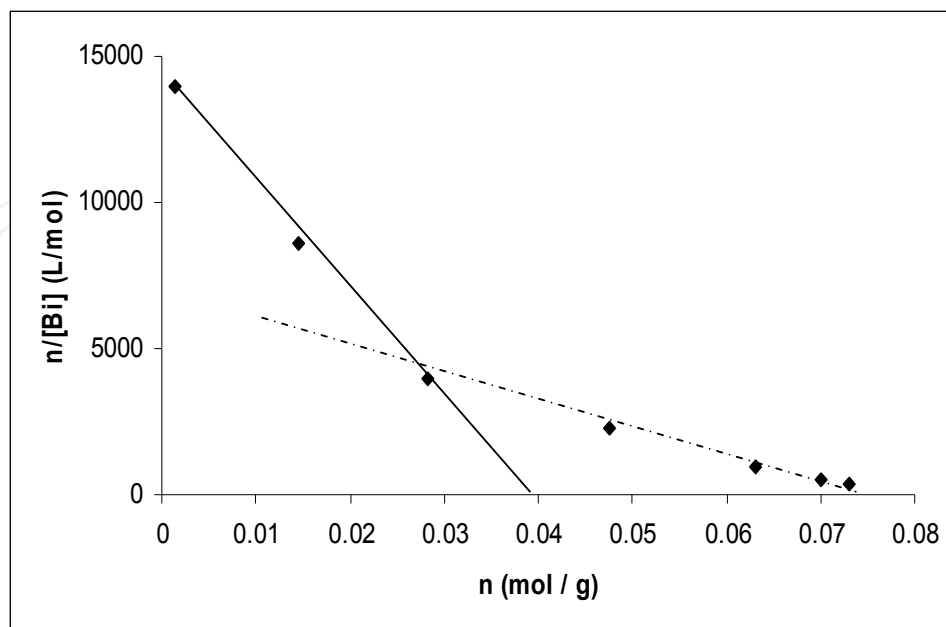
Figure 3. Scatchard plot for the binding of [\text{BiI}_4]^- species by \text{PQ}^+ \cdot \text{Cl}^- immobilized PUF ( 0.1 \pm 0.002 \text{ g} ) from aqueous media containing KI (10 % m/v) - \text{H}_2\text{SO}_4 ( 0.5 \text{ mol L}^{-1} ) at 25 \pm 0.1^\circ\text{C} .
