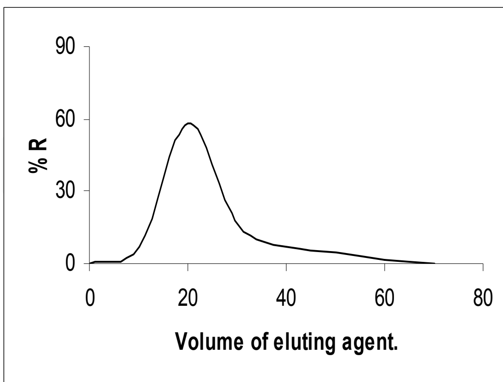
Figure 14. Chromatogram of bismuth (III) recovery from PQ+.Cl - loaded PUFs packed column using nitric acid (5 mol L -1 ) as eluting agent at flow rate of 2.5 mL min -1 .
