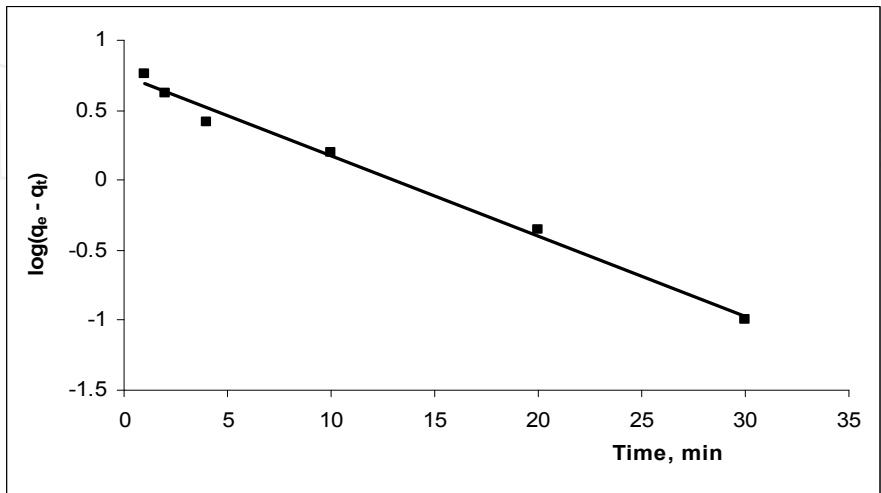
Figure 5. Lagergren plot of bismuth (III) uptake onto PQ + .Cl - PUFs from aqueous solutions containing KI (10 % m/v) - H 2 SO 4 (2.0 mol L -1 ) vs. time at 25 ± 0.1°C. ]
