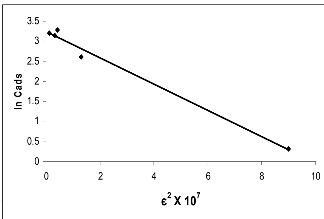
Figure 13. Dubinin-Radushkevich (D-R) sorption of bismuth (III) extraction from aqueous solution onto \text{PQ}^+\text{Cl}^- loaded PUFs at the optimum conditions
