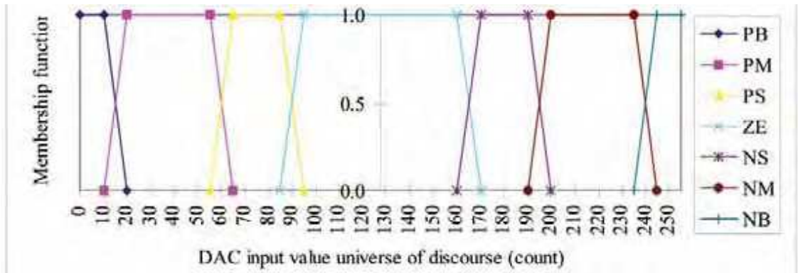
Figure 14. Control action fuzzy set definition.
