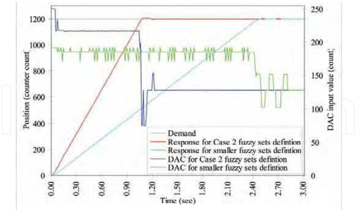
Figure 20. Waist response for different tuned fuzzy sets at second robot arm configuration.
