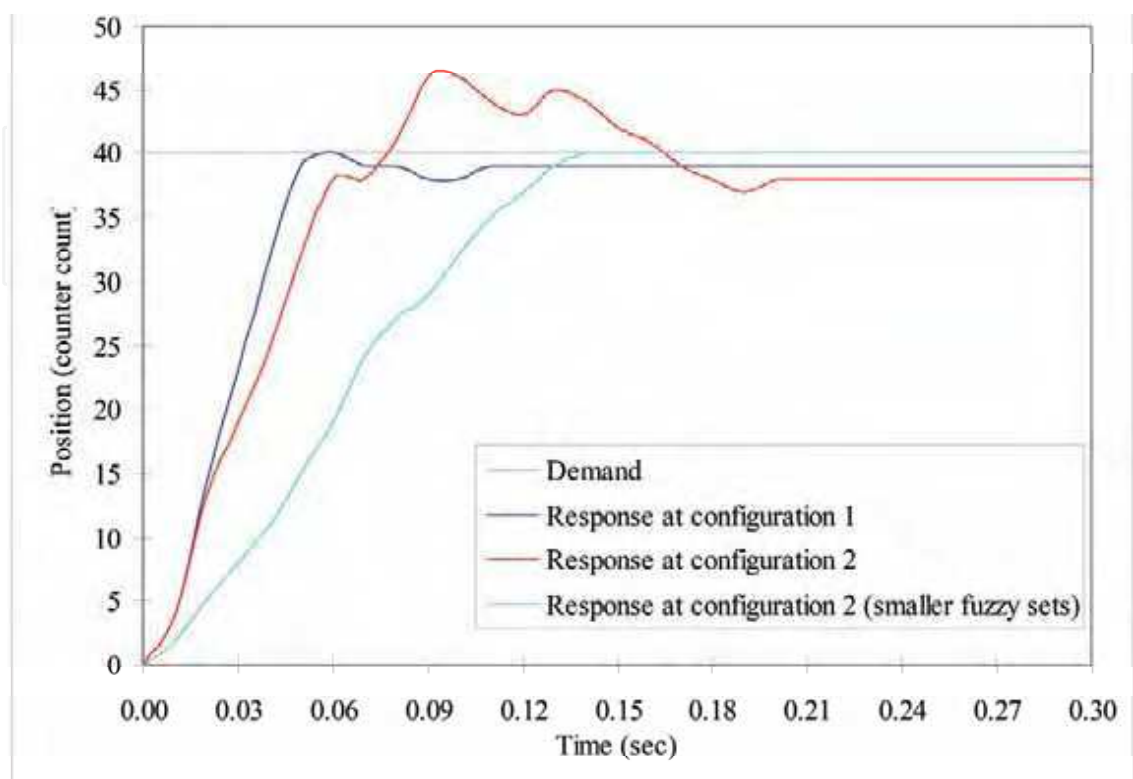
Figure 16. Waist response at different arm configurations.
