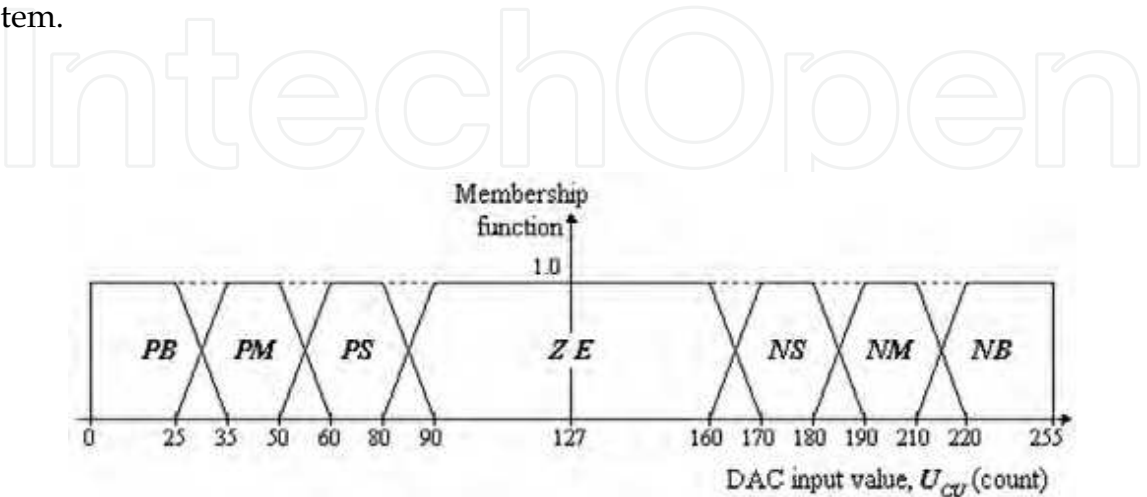
Figure 4(b). Control action domain of discourse
