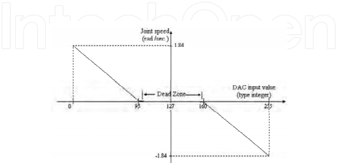
Figure 4(a). A typical characteristic for the waist joint actuator
