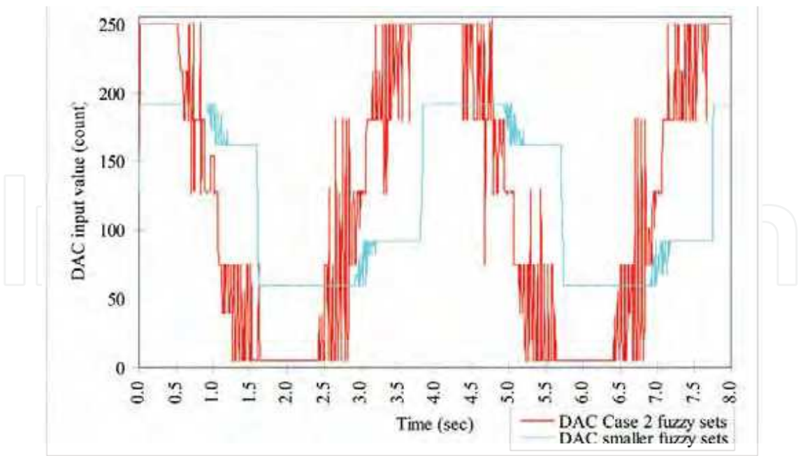
Figure 21(b). Control signal in Fig. 21(a).
