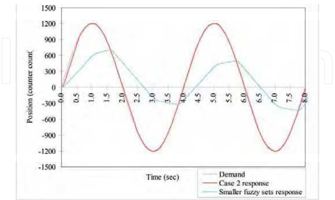
Figure 21(a). Response of the smaller and Case 2 fuzzy set combinations to sinusoidal tracking.
