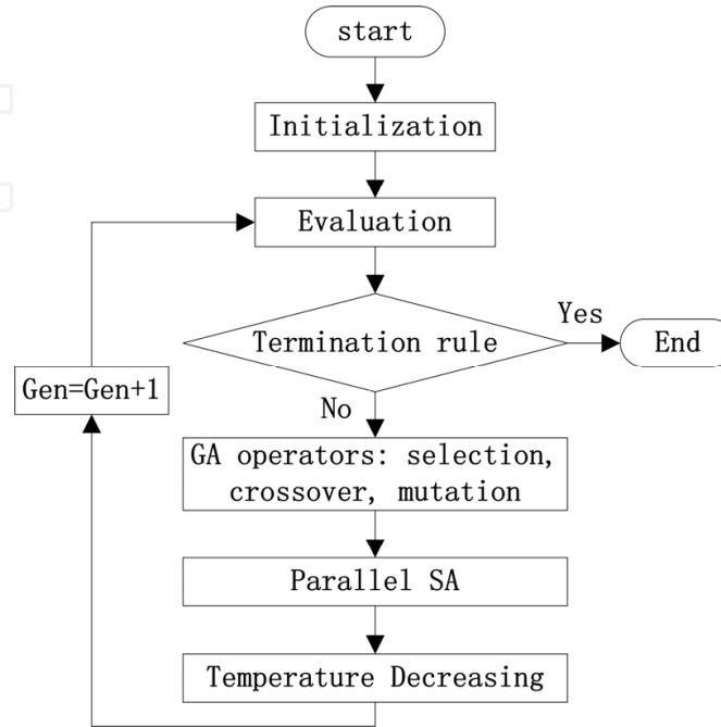
Figure 1. Flow chart of the implemented GA-SA
