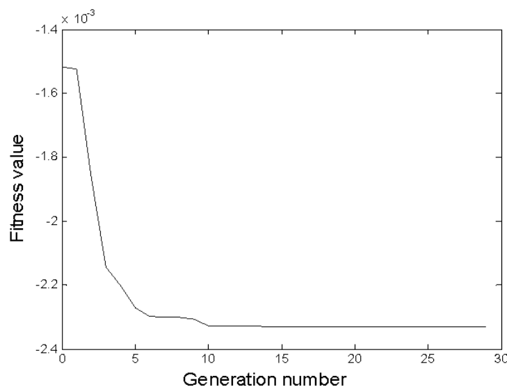
Figure 5. Convergence of the GA-SA algorithm
