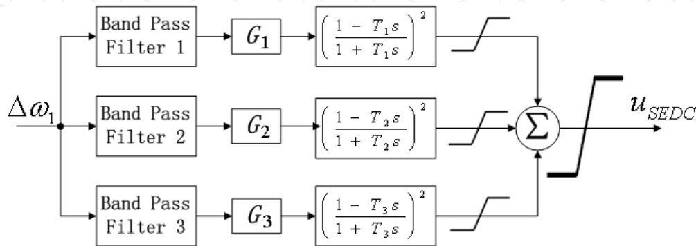
Figure 4. Configuration of SEDC
