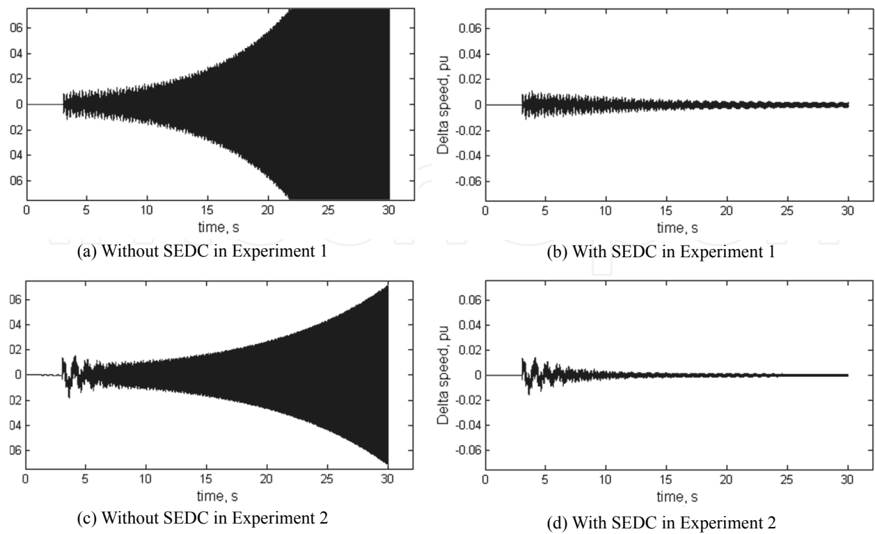
Figure 6. Delta mechanical speed of the high-pressure turbine
