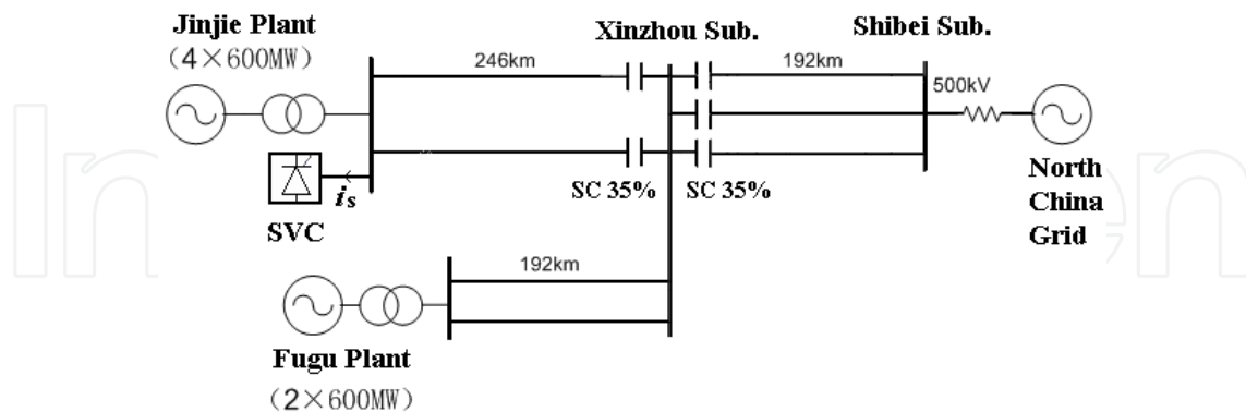
Figure 9. The one-line diagram of the equivalent transmission system
