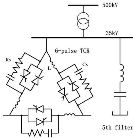
Figure 10. The power-electronic circuit of the six-pulse SVC
