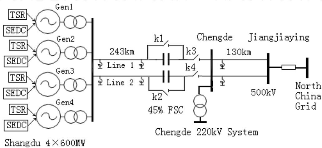
Figure 2. The one-line diagram of the equivalent transmission system
