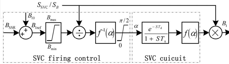
Figure 11. The dynamic model of the SVC
