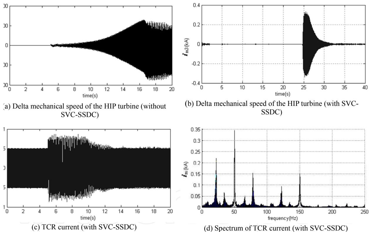
Figure 15. System response following a three-phase fault
