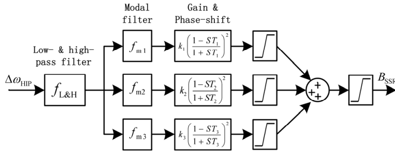
Figure 12. Configuration of SVC-SSDC
