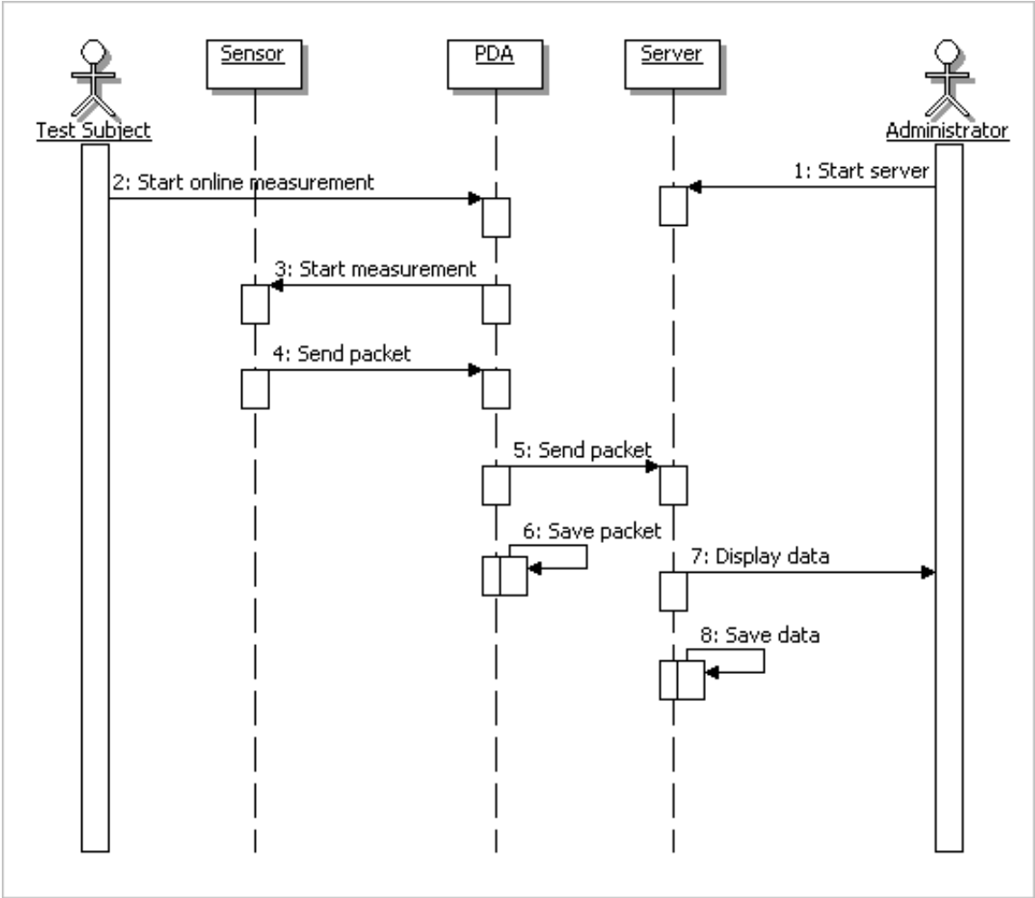
Figure 5. The Overall System Sequence Diagram
