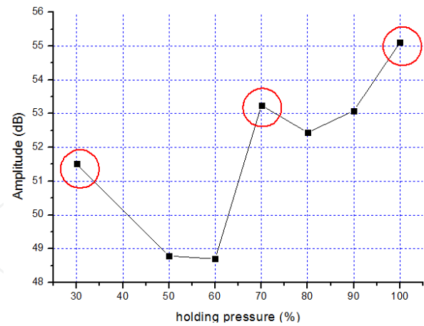
Figure 9. Mean amplitude during load holding
