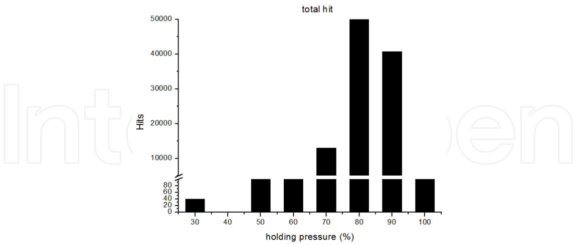
Figure 6. Total hits during load holding
