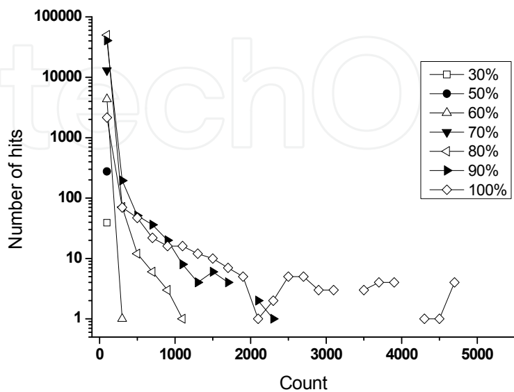
Figure 14. Count distribution during load holding
