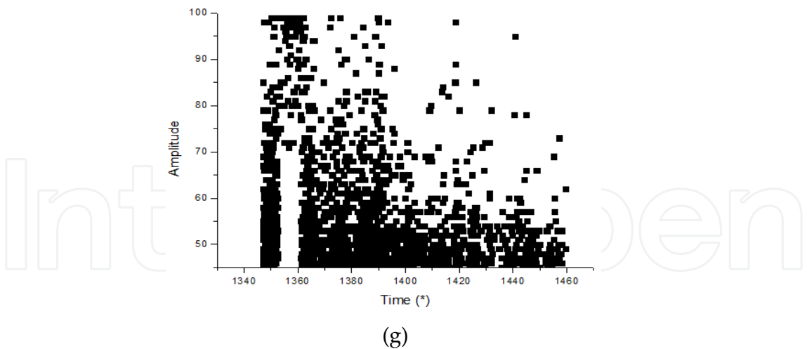
Figure 5. Amplitude vs Time plot during load holding : (a)30% (b)50% (c)60% (d)70% (e)80% (f)90% and (g)fractured
