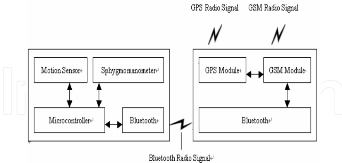
Figure 5. Tele-emergency announcement system architecture
