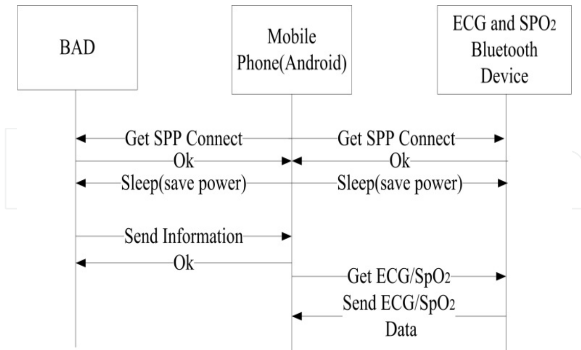
Figure 22. System communication
