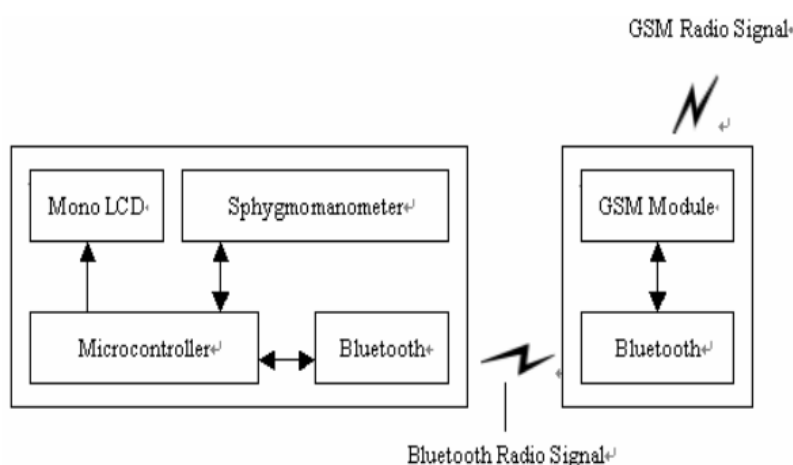
Figure 4. Tele-care system architecture
