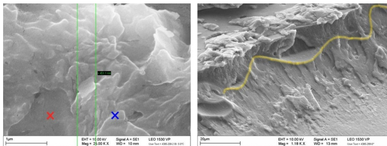
Figure 10. Sections of impact crater produced from single spherical impacts at 273K. Fracture surfaces of the primer layer are shown. Left image shows the composite of Fig. 9., scale bar is 1 μm. Tortuous cracking took place in the rigid composite leaving individual LDH stacks behind. Right image is a stratified primer (yellow line = interface) comprising aggregated carbonated LDH particles in the layer beneath the upper PURh phase, scale bar is 20 μm.
