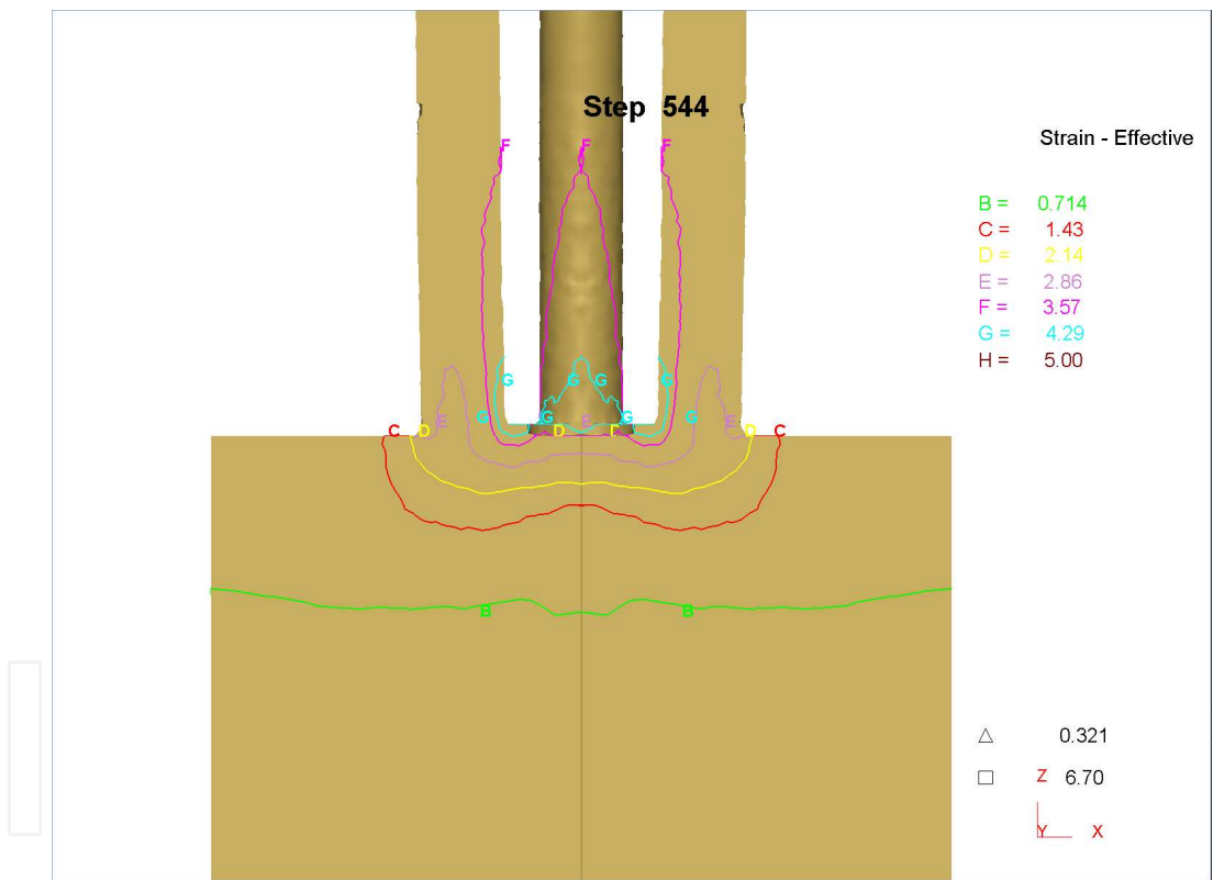
Figure 10. Distribution of intensive strain upon extrusion through ring-shaped pocket die.
