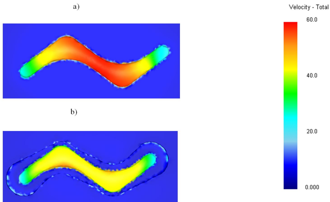
Figure 19. Distribution of metal exit velocity in the die orifice in case of, a) flat die, b) pocket die.
