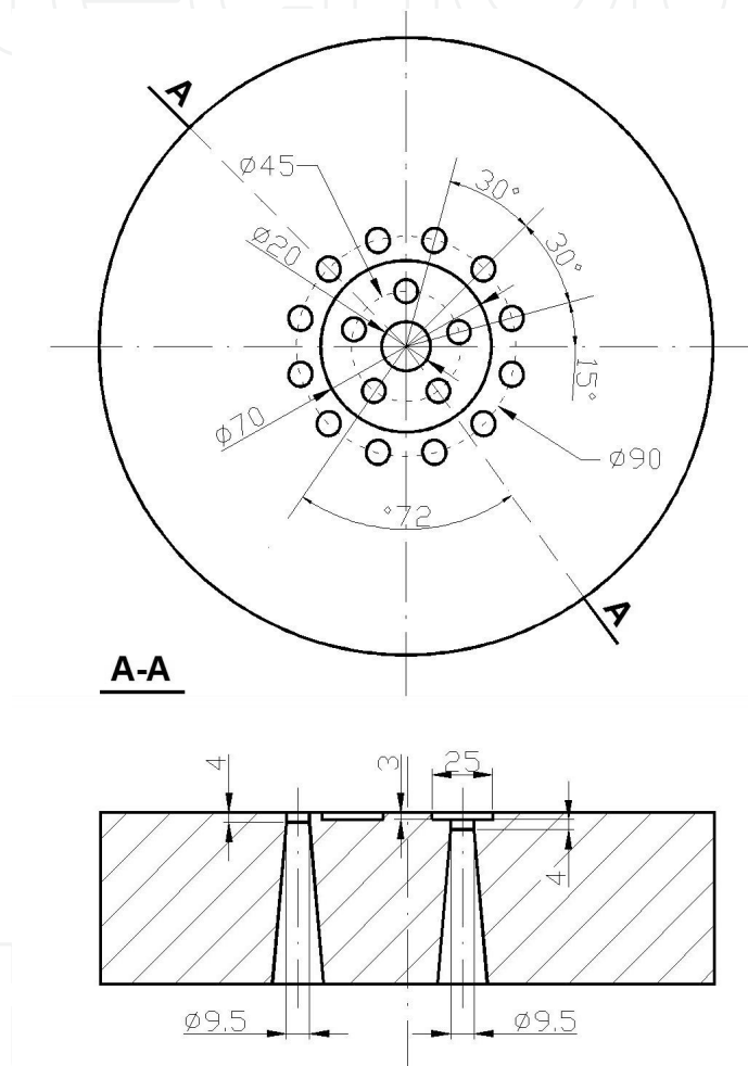
Figure 12. Schematic diagram of 17-hole die with ring-shaped pocket, dimensions in mm.
