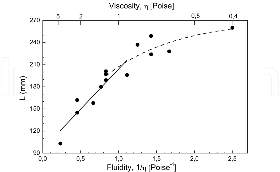
Figure 12. Slag ribbon length ( L ) as a function of fluidity ( 1/\eta ).
