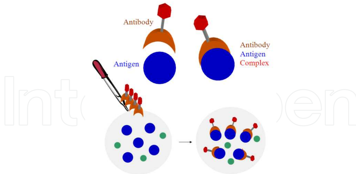
Figure 6. Antigens, like GAD 65, are detected by specific capturing with their corresponding antibodies. This enables it to pick up the antigen GAD 65 from a mixture of molecules.
