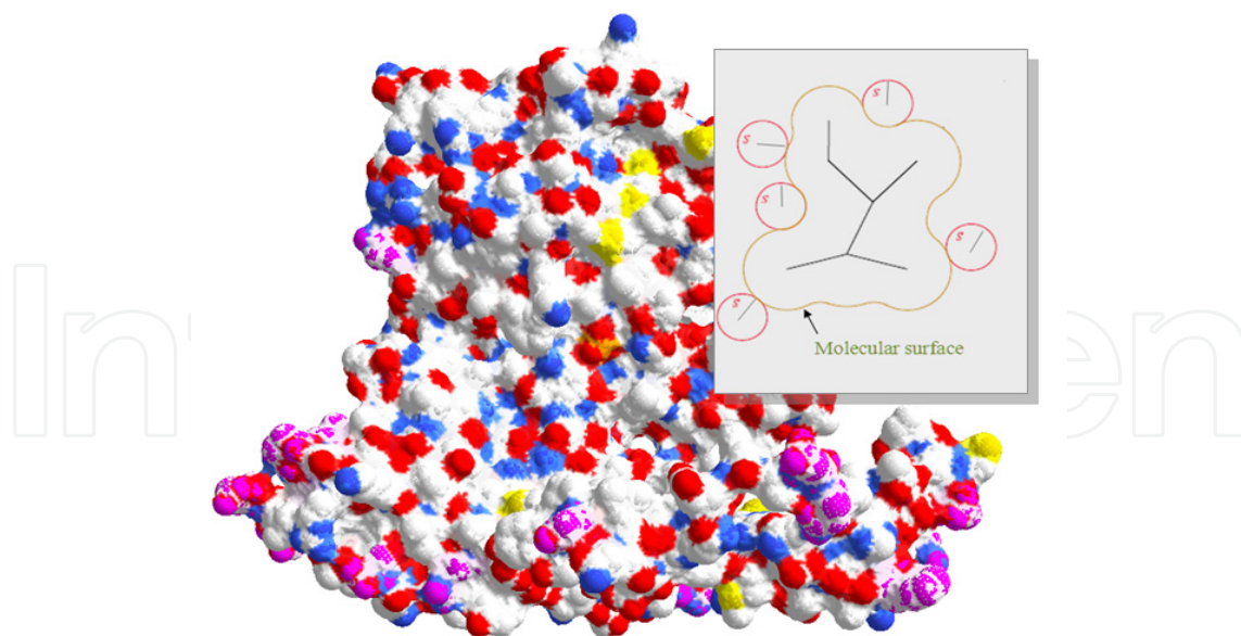
Figure 20. Molecular surface of GAD 65: Boundary that is obtained by rolling the solvent sphere over the van der Waals surface. The molecular surface is the envelope generated by the rolling sphere. It consists of sphere and torus patches connected in a tangent continuous manner and filling up the inaccessible crevices and cusps.
