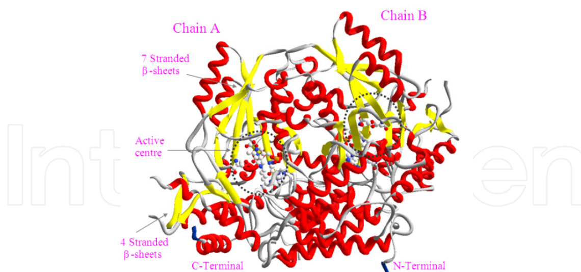
Figure 5. The enzyme GAD 65 is a dimer. Each chain contains 4 stranded \beta -sheets (yellow) surrounded by three \alpha -helices (red) and 7 stranded \beta -sheets surrounded by eight \alpha -helices. Every chain has an own active centre.
