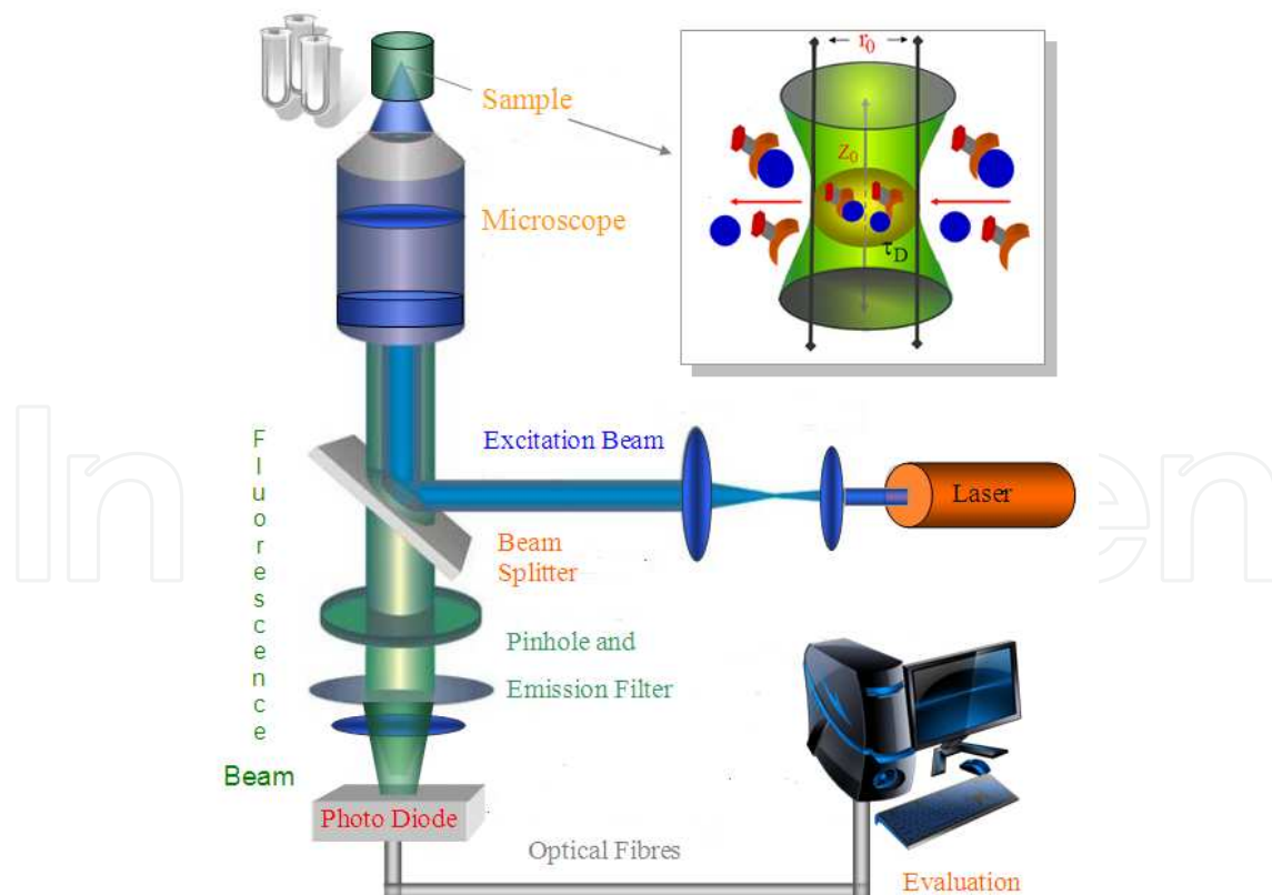
Figure 7. Set up and principle of the Fluorescence Correlation Spectroscopy (the radius r_0 is approximately 0.5 \mu\text{m} ).
