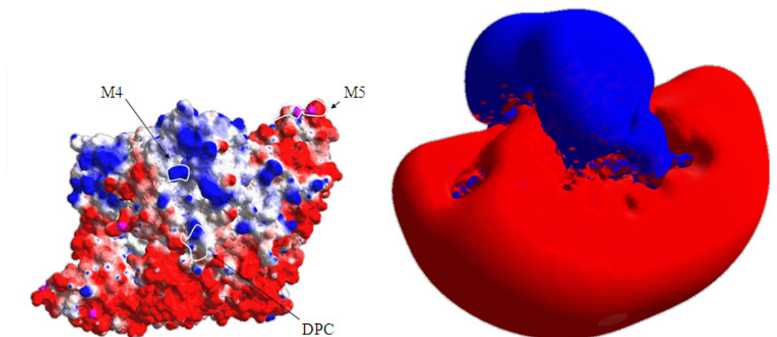
Figure 27. The electrostatic potential surrounding the GAD 65 molecule plays an important role in the specific antibody recognition. The electrostatic potential map shows contours of constant values. Positive potential values are drawn in blue, negative values in red. Different constant electrostatic potential values, ranging from the neighbourhood (left) to more extended ranges (right) are shown.
