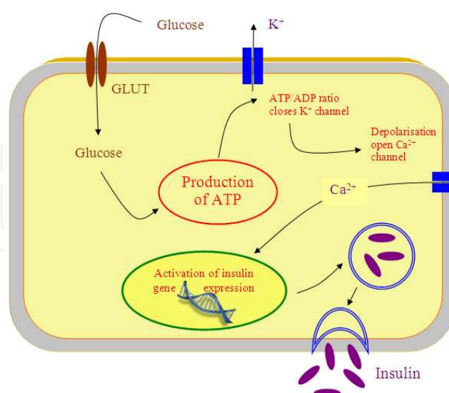
Figure 1. By the decomposition of glucose, ATP is produced in the beta cells. The increase of the ATP concentration closes the K + channel, leading to a depolarisation which in consequence opens the Ca 2+ channel. Ca 2+ activates the insulin gene expression via the Calcium Responsive Element Binding Protein (CREB). By exocytosis, the produced insulin is set free in the blood.
