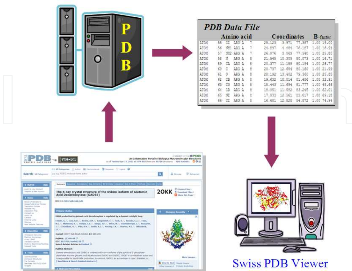
Figure 17. Protein structural information is available at the Protein Data Base (PDB). At the moment the database contains more than 80.700 experimentally determined structures. The PDB is contacted through the Internet. The structural information is stored in the PDB data files as atomic coordinates. The B-factor indicates the precision of each atom position. The requested PDB data files are downloaded and the protein structure visualized locally.
