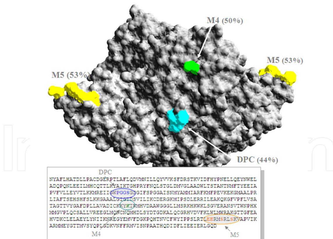
Figure 21. The GAD 65 molecule is represented by its molecular surface. The shapes of the GAD 65 epitopes, enable a pictorial analysis of the local docking sites. The exposure values of the residues, constituting the epitopes, were calculated by Voronoi tessellation. These values (in %) indicate how much the epitopes are exposed to the surrounding solvent, indicating the accessibility to potential antibodies.
