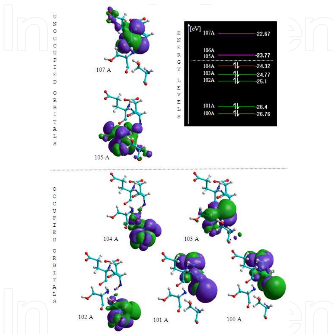
Figure 24. A subset of the molecular orbitals from the epitope M5 is shown together with their energy levels. Positive values of the molecular orbitals are green encoded, negative values violet. The most important orbitals in organic chemistry are the highest occupied molecular orbital (HOMO: 104 A) and the lowest unoccupied molecular orbital (LUMO: 105 A).
