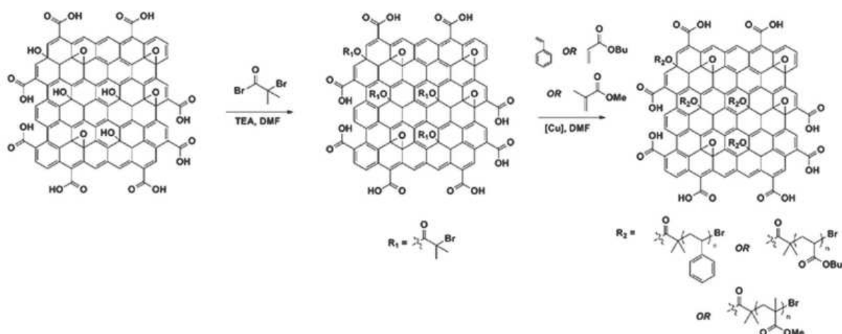
Figure 1. Synthesis of surface-functionalized GO via attachment of an ATRP initiator ( \alpha -bromoisobutyryl bromide) followed by polymerization of styrene, butyl acrylate, or methyl methacrylate [38].
