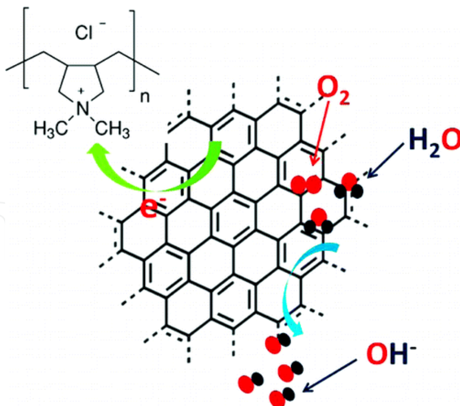
Figure 22. Schematic illustration of the electron-withdrawing from graphene by PDDA to facilitate the ORR process [97].
