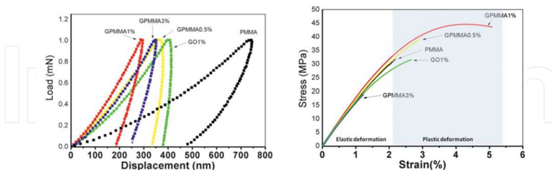
Figure 3. Load-displacement nanoindentation (left) and stress-strain curves (right) of films of PMMA and its nanocomposites with PMMA-functionalized graphene. 40
