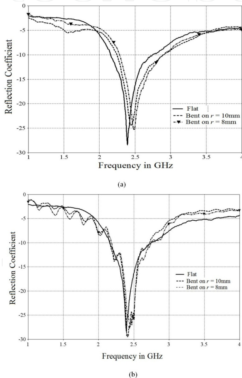
Figure 14. Measured S_{11} for the reported antenna when bent on a foam cylinder with different radii ( r=10\text{ mm} and r=8\text{ mm} ) to mimic different bending extents. (a) horizontal plane, (b) vertical plane.
