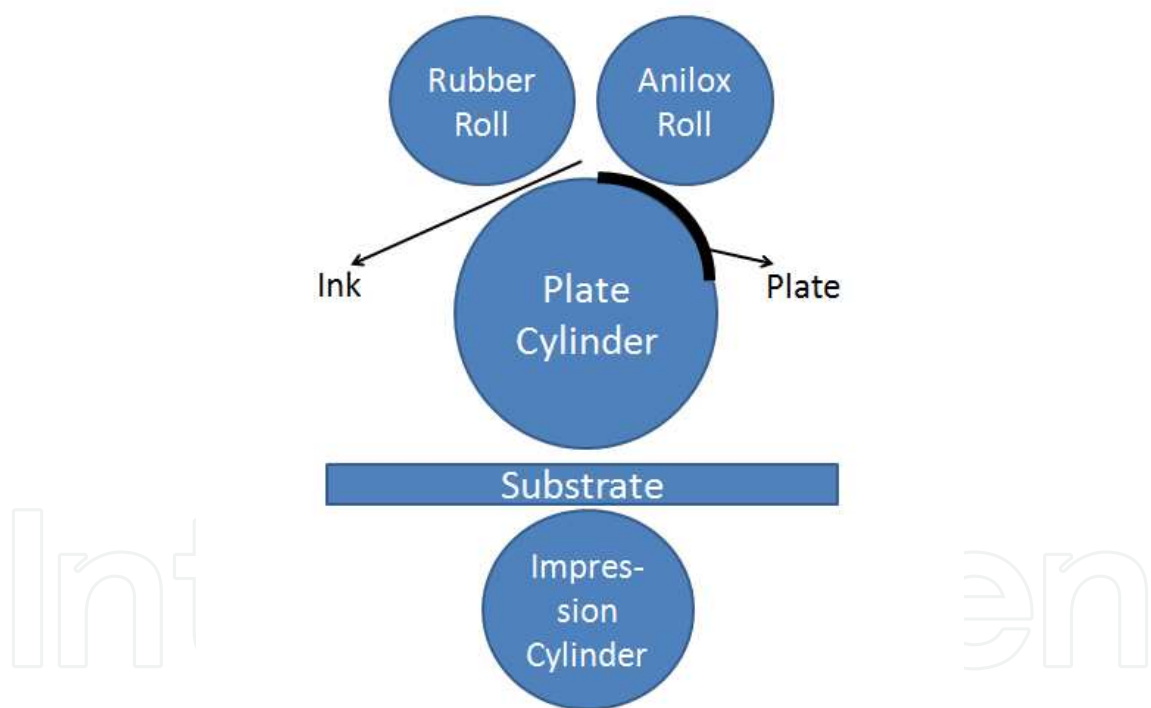
Figure 4. Illustration of the flexography printing process based on flexible relief plate.
