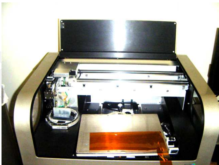
Figure 8. Installing the polyimide substrate on the platen of the material printer.
