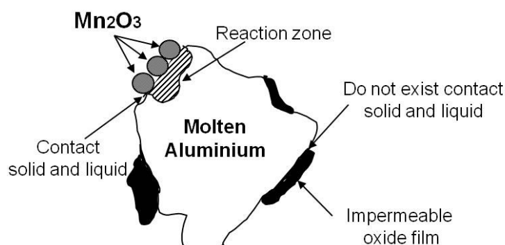
Figure 1. Scheme of the aluminothermic reduction of \text{Mn}_2\text{O}_3 [10,11].
