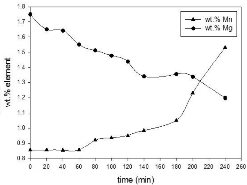
Figure 8. Variation of the concentrations of Mn and Mg, with respect to treatment time, during the metallothermic reduction of \text{Mn}_2\text{O}_3 , for a target Mn concentration of 1.50 wt. % at constant temperature.
