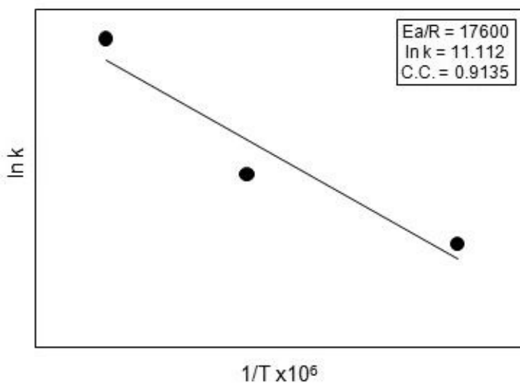
Figure 11. Linear plot of \ln k vs 1/T , for determining the activation energy in the aluminothermic reduction of \text{Mn}_2\text{O}_3 .
