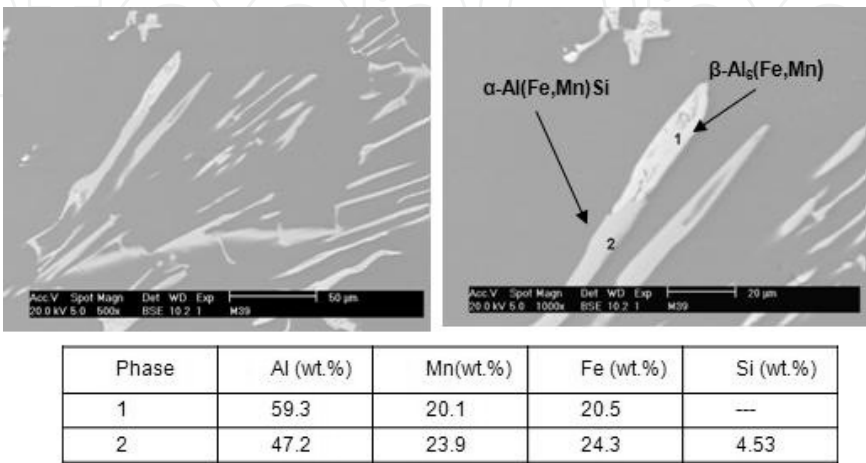
Figure 15. SEM micrograph of an Al-1 wt. %Mn alloy showing the morphology of the \beta-Al_6(Fe,Mn) and \alpha-Al_{12}(Fe,Mn)_3Si phases particles after a homogenizing treatment at 550^\circ C for 15 hours.
