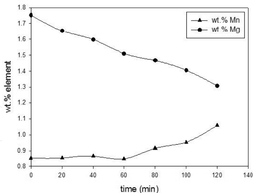
Figure 5. Variation of the concentrations of Mn and Mg, with respect to treatment time, during the metallothermic reduction of \text{Mn}_2\text{O}_3 , for a target Mn concentration of 1 wt. % at constant temperature.
