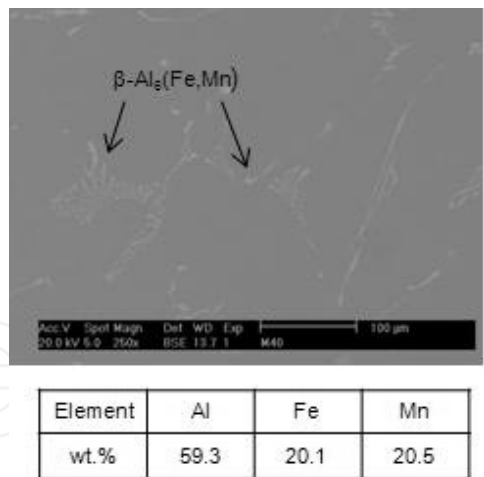
Figure 14. Micrograph obtained by SEM showing the morphology of the particles of the \beta\text{-Al}_6(\text{Fe,Mn}) phase, in anal- loy Al-1 wt. % Mn in the as cast condition.
