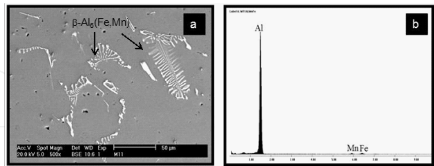
Figure 13. SEM micrograph showing the morphology of: a) \beta\text{-Al}_6(\text{Fe,Mn}) : EDS pattern of the Mn rich particles, in an alloy with a final concentration of 1 wt. %Mn.
