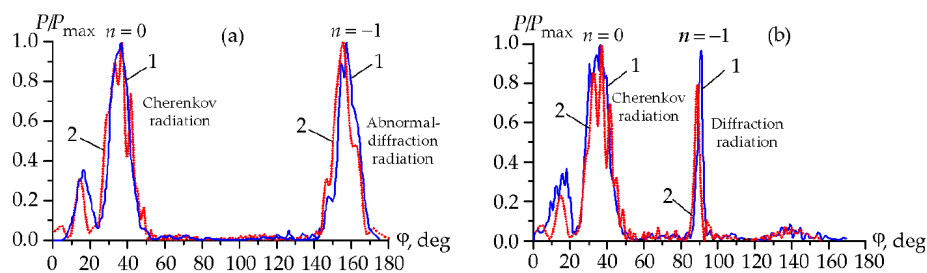
Figure 2. Typical directional radiation patterns of spatial waves on the MDS: (a) Cherenkov and abnormal-diffraction modes; (b) diffraction-Cherenkov mode. 1 — experiment, 2 — numerical simulation.
