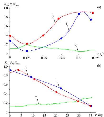
Figure 7. Amplitude and waveguide characteristics of the PD with (a) longitudinal and (b) angular shifts of grid bars with respect to the axis of the waveguide. 1 — relative power values P_3 , 2 — K_{tr} values, 3 — calculated curve.
