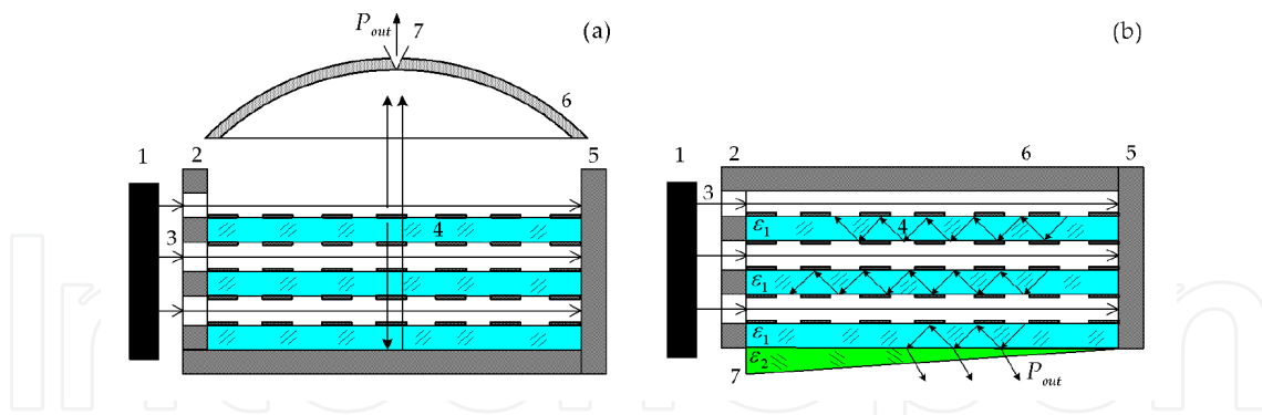
Figure 13. Schematic view of low voltage vacuum devices employing multi-linked MDS: (a) orotron, (b) backward wave oscillator. 1 — cathode, 2 — anode, 3 — EB, 4 — planar periodic MDS, 5 — collector, 6 — mirror, 7 — output port.
