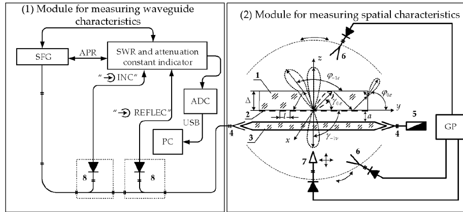
Figure 1. Block diagram of the experimental setup: (SFG) sweep-frequency generator, (APR) automatic power regulator, (ADC) analog-to-digital converter, (PC) personal computer, (GP) two-coordinate graph plotter. 1 — dielectric prism, 2 — strip DG, 3 — DW, 4 — matching junctions, 5 — matched load, 6 — horn antenna, 7 — probe, 8 — (DC) directional couplers, \gamma — radiation angles of the MDS-DW system, \varphi — angles of corresponding radiation harmonics in the free space after transmission through the dielectric prism, x , y , and z — spatial coordinates, \Delta — thickness of the dielectric layer, a — distance between the DW and strip grating 2 (aiming parameter).
