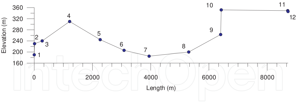
Figure 14. Elevation and length profile of Espite pipeline
