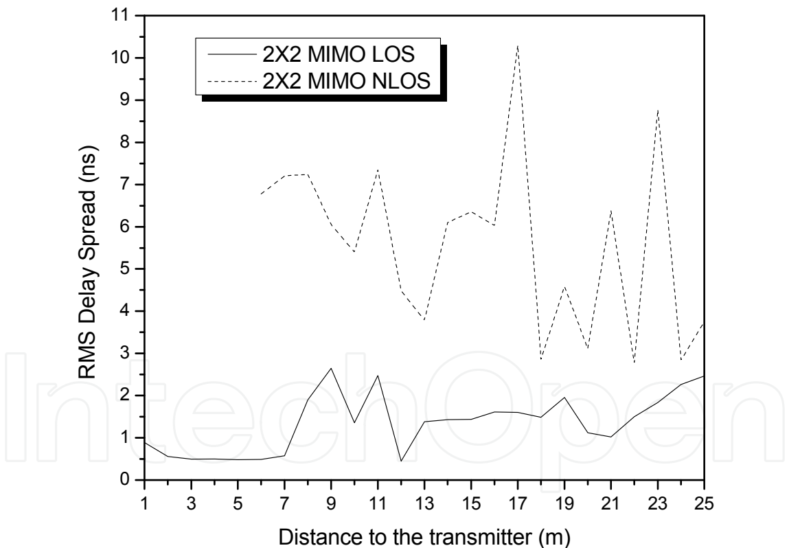
Fig. 15. RMS delay spread as a function of the distance
