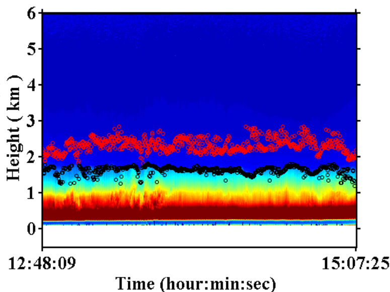
Fig. 14. Height-Time-Color map of LIDAR signal returns (arb.unit) for 27 May 2011. The figure is overlapped by the determined boundary layer height (Black: statistical method based on range corrected signal, Pink: slope method)
