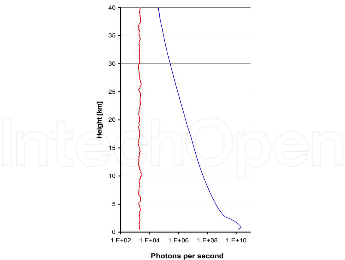
Fig. 11b. Height profile of averaged photon count for the above presented temporal evolution in fig. 11a.
