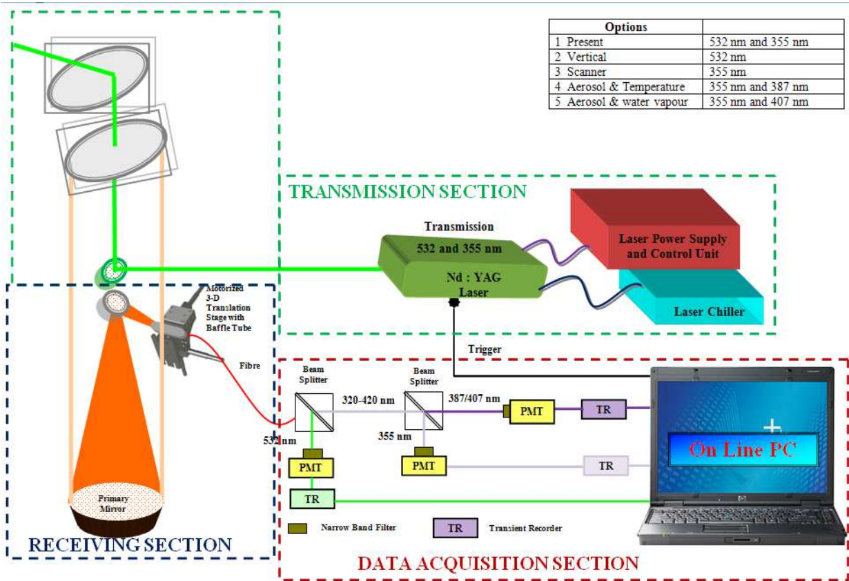
Fig. 4. Block diagram of CSIR-NLC mobile LIDAR illustrating different components.
