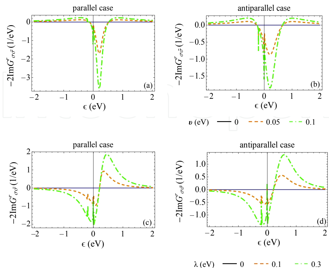
Fig. 6. (a),(b): Off-diagonal spectral functions as a function of energy, for varying SF-TJ strength ( v ) between leads and QD, in the absence of SF-QD (i.e., \lambda = 0 eV). (c),(d): Off-diagonal Spectral functions as a function of electrons' energy, with varied SF-QD strength ( \lambda ), in parallel (left) and antiparallel (right) case, where v = 0 eV. Other parameters are the same with those in Fig. 3.
