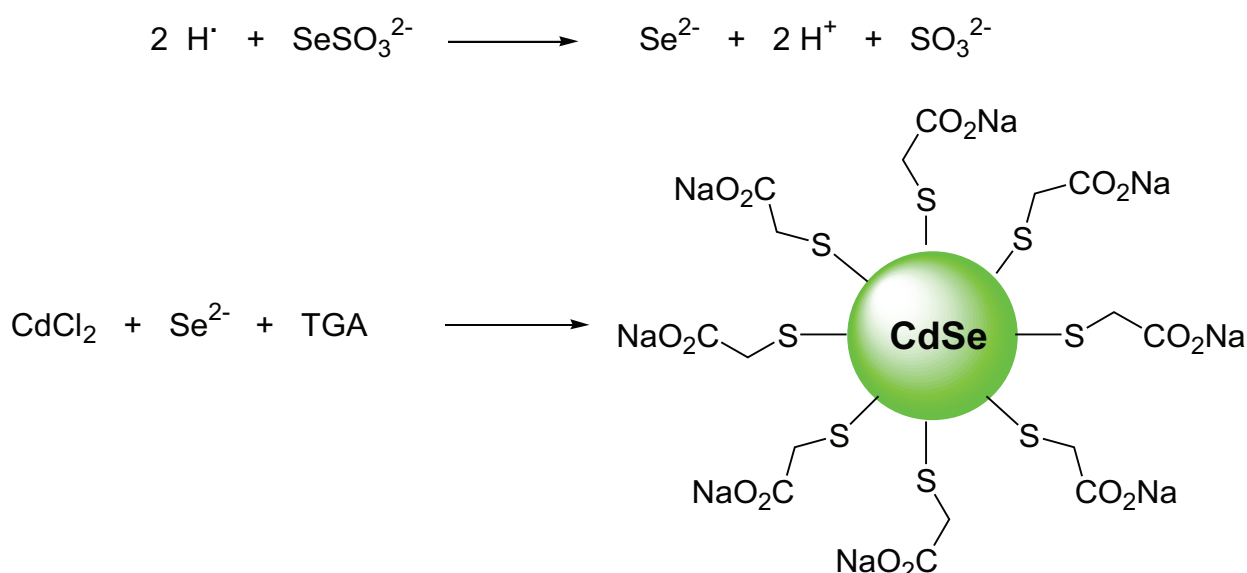
Fig. 17. Synthesis of CdSe@TGA QDs under ultrasonic irradiation
