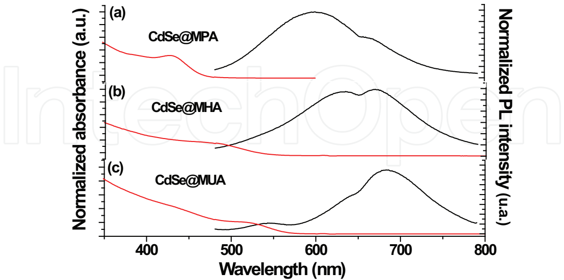
Fig. 19. UV-vis absorption (red) and PL (black) spectra of (a) MPA-, (b) MHA- and, (c) MUA-stabilized CdSe QDs prepared at 100°C for 15 h. PL spectra were recorded with an excitation at 400 nm.
