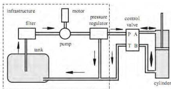
Fig. 8. Major Components of Hydraulic System
