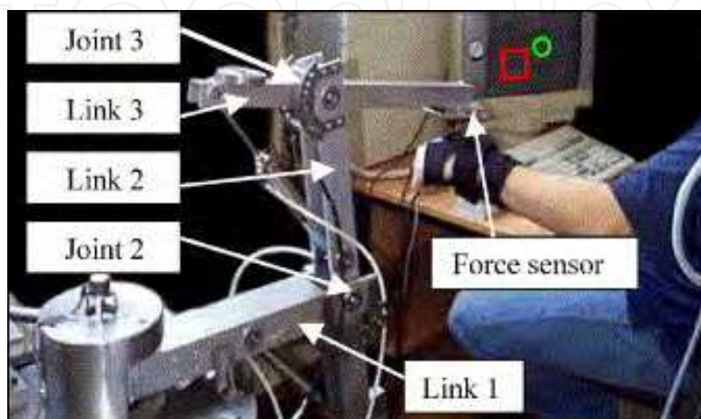
Fig. 26. 3-DOF pneumatic actuated device. (Richardson et al., 2003)
