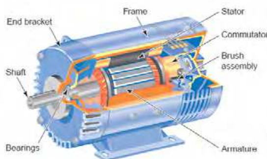
Fig. 5. Major Components of DC Motor (Petruzella, 2010)
