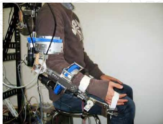
Fig. 21. SUEFUL-7 ( http://www.me.saga-u.ac.jp/~kiguchi/research_en.html#research01 , December 2011)
