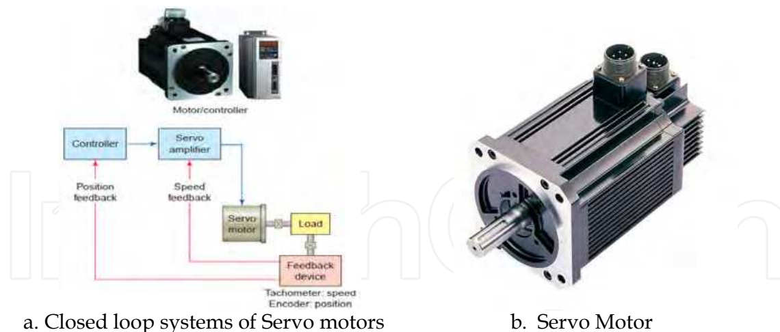
Fig. 6. Closed loop systems of servo motors and servo motor (Petruszella, 2010)
