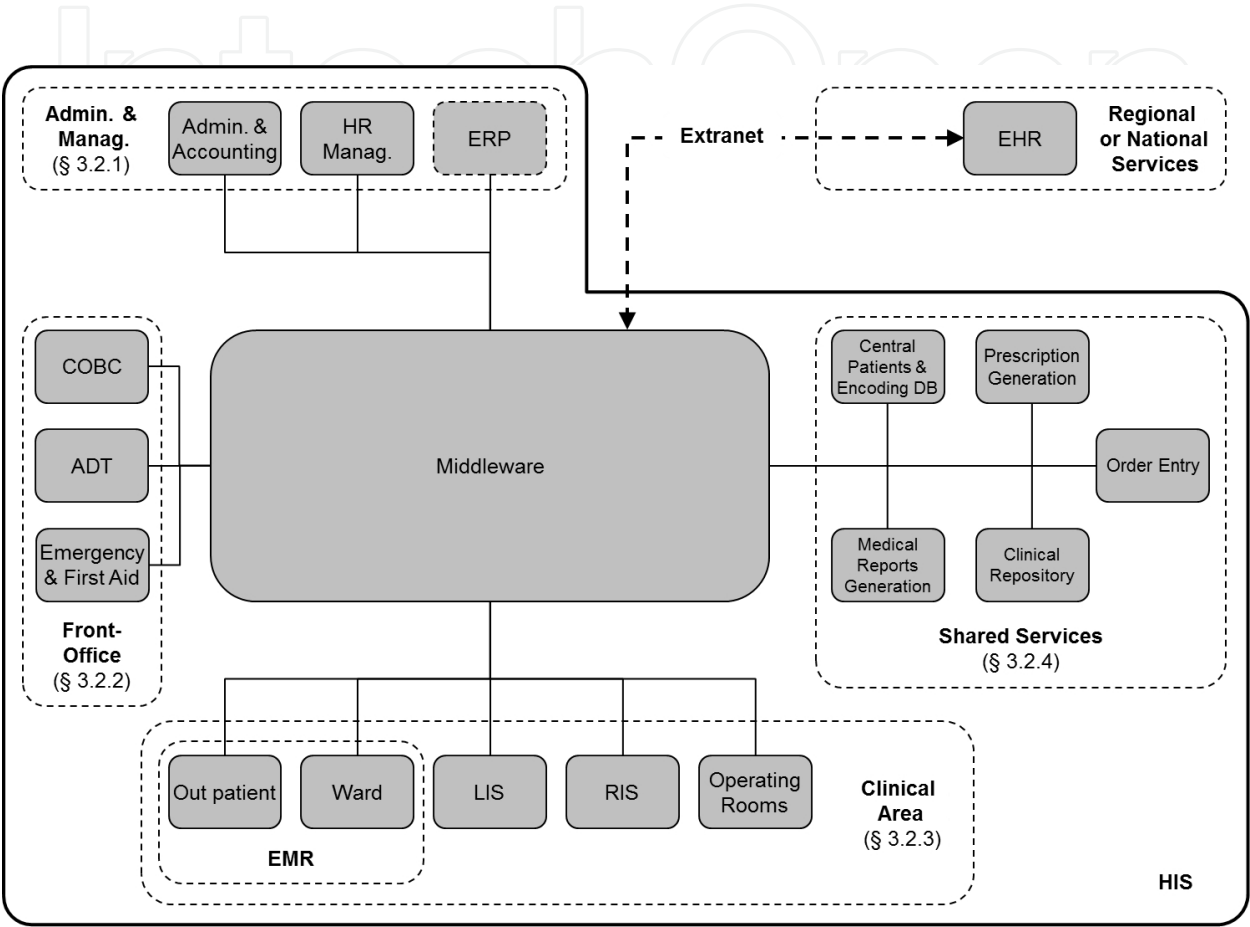
Fig. 1. Conceptual Architecture of a HIS
