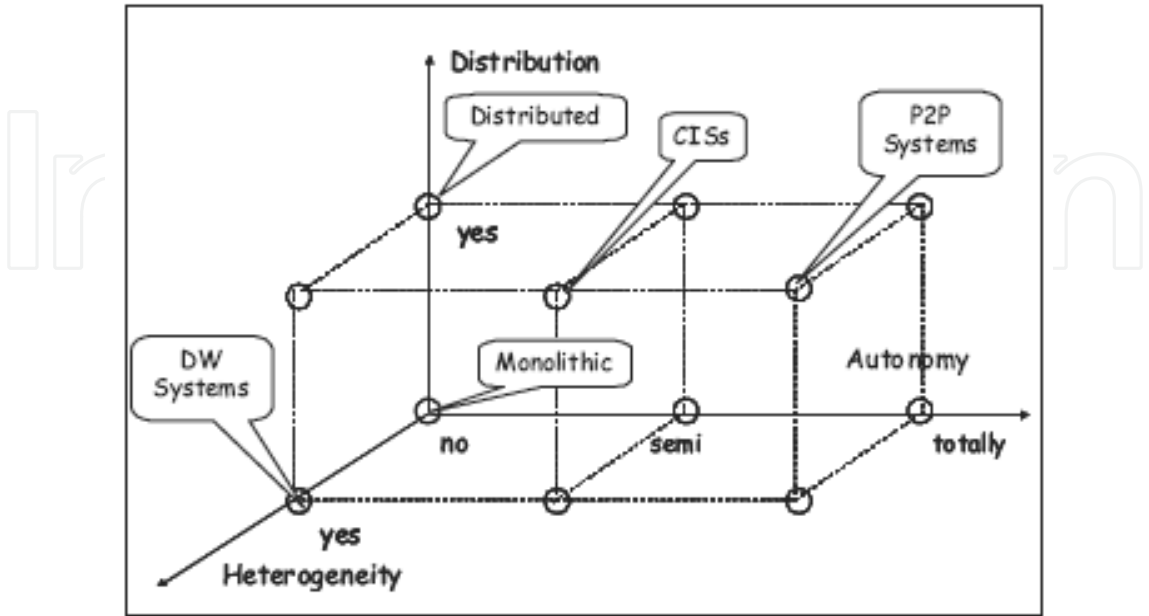
Fig. 2. Type of Information Systems (Batini&Scannapieco, 2006)
