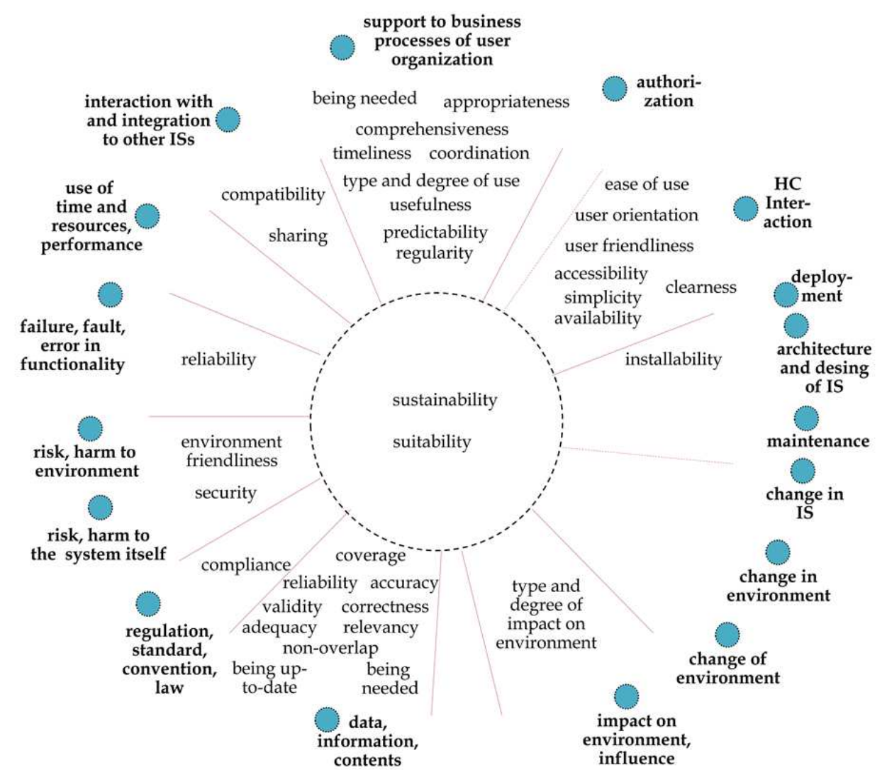
Fig. 7. An example of domain-attribute set
