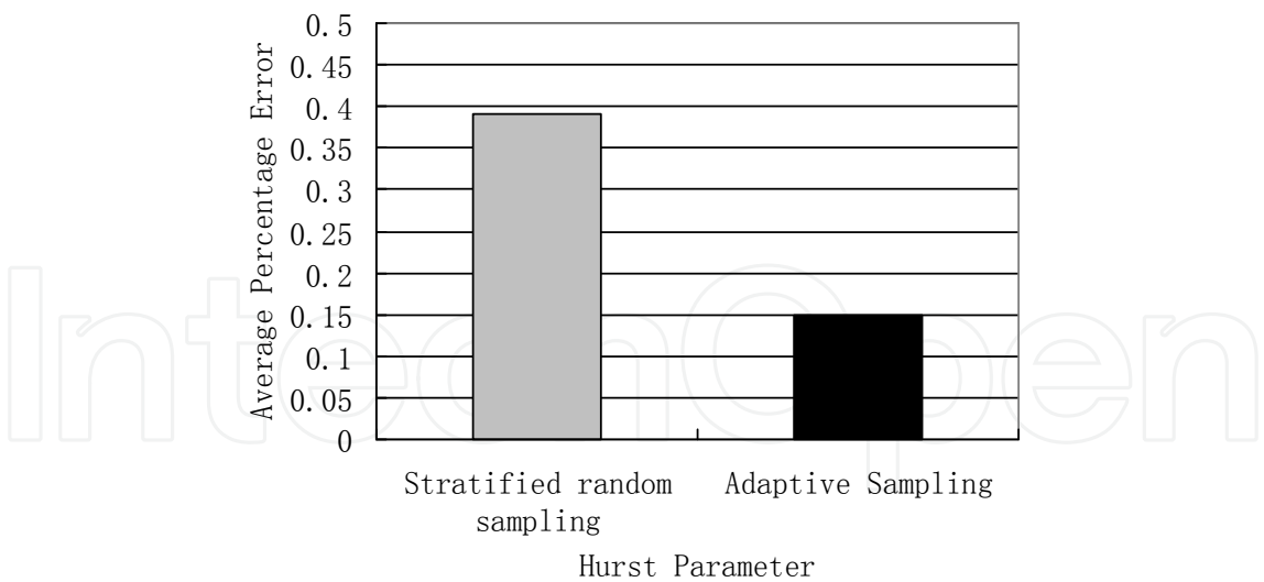
Fig. 13. Average percentage error for the Hurst parameter.
