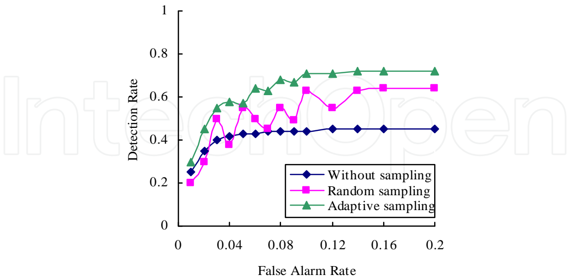
Fig. 16. The ROC curves at a 10-Gbps speed.
