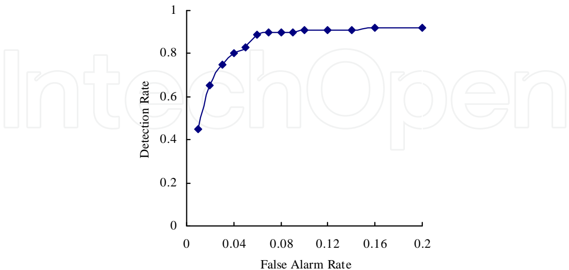
Fig. 15. The ROC curves at 1-Gbps speed.
