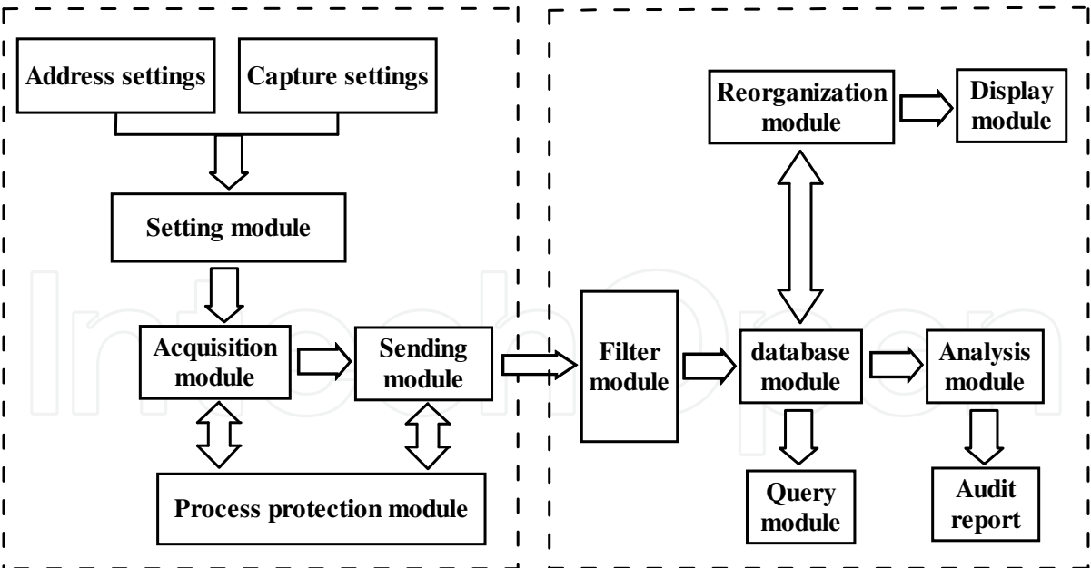
Fig. 3. Architecture of Security Audit System
