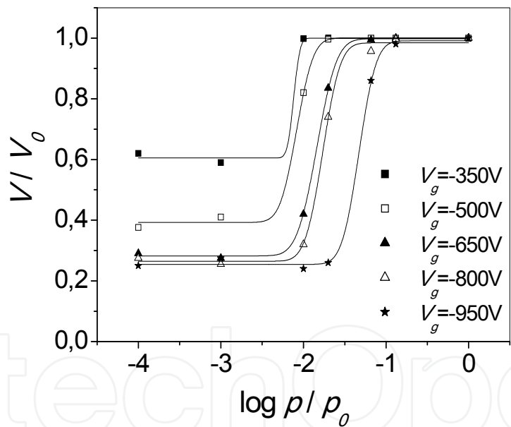
Fig. 9. Dependence of the normalized surface potential on the normalized pressure for negatively charged PP samples at 90°C. Infinite air gap.
