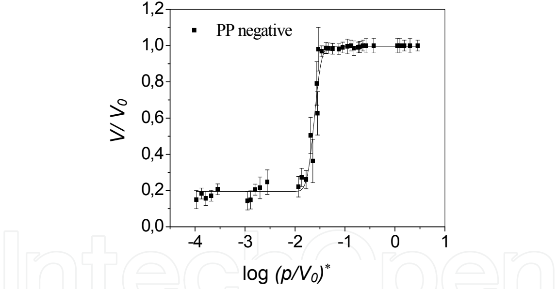
Fig. 20. Dependence of the normalized surface potential V / V_0 on the normalized ratio (p/V_0)^* for negatively charged PP samples.
