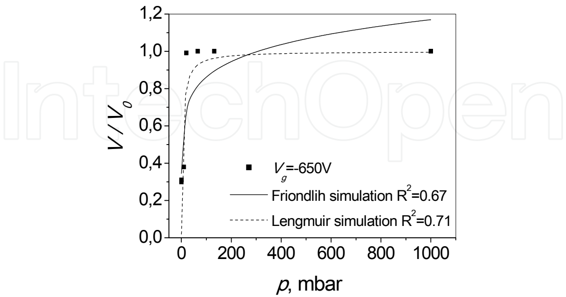
Fig. 15. Dependence of the normalized surface potential on pressure for PP samples charged in negative corona, at 20°C fitted by the Friondlih and Lengmuir equations. Infinite air gap.
