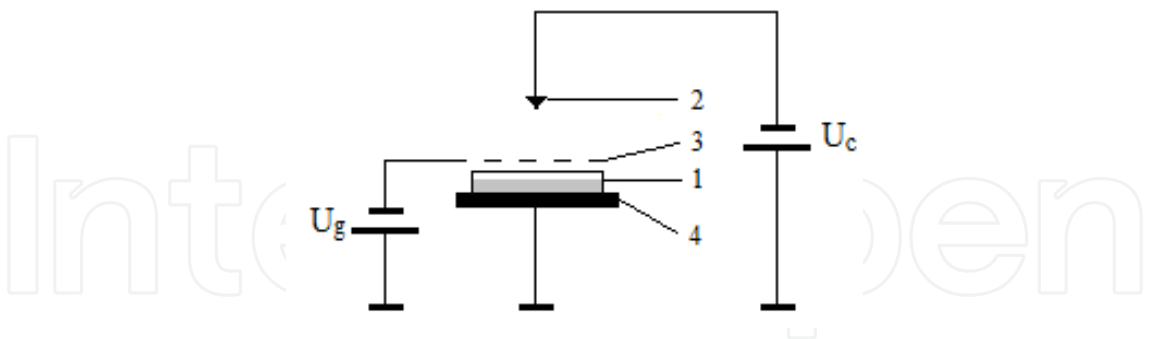
Fig. 1. Arrangement of the corona charging set-up. 1 – sample on a metal pad; 2 – corona electrode; 3 – grid; 4 – grounded plate electrode; U_g – grid voltage power supply; U_c –corona voltage power supply.
