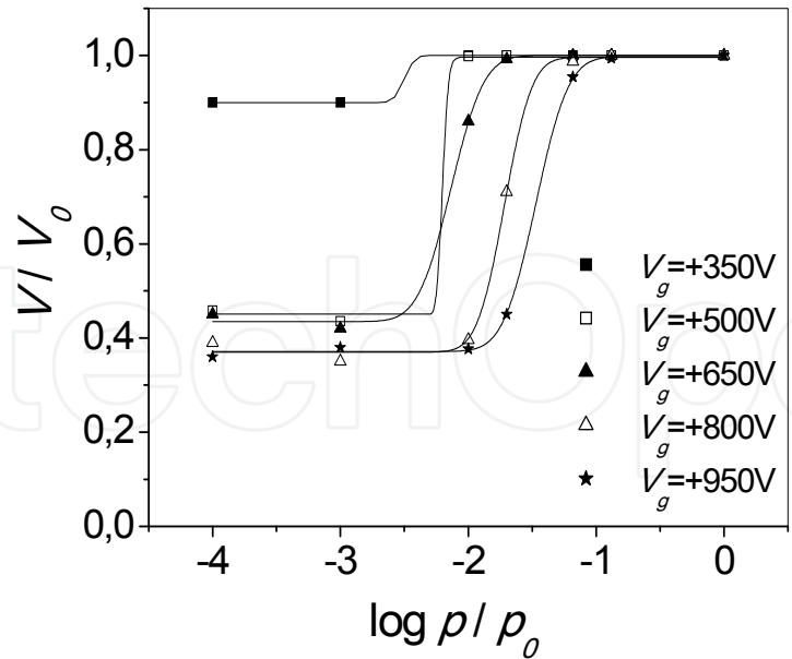
Fig. 8. Dependence of the normalized surface potential on the normalized pressure for positively charged PP samples at 90°C. Infinite air gap.
