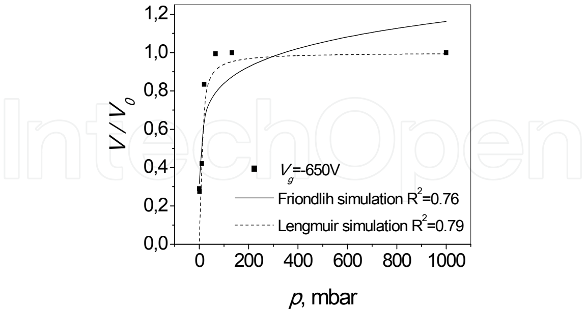
Fig. 16. Dependence of the normalized surface potential on pressure for PP samples charged in negative corona at 90°C, fitted by the Friondlih and Lengmuir equations. Infinite air gap.
