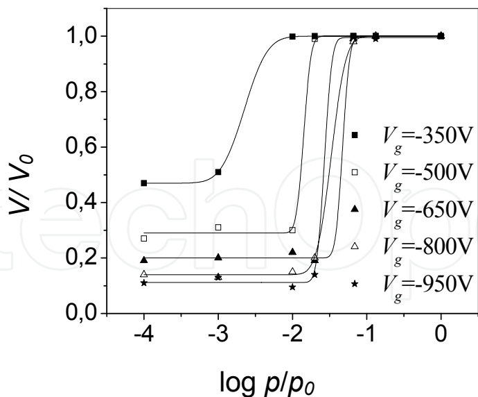
Fig. 5. Dependence of the normalized surface potential on normalized pressure for negatively charged PP samples. The air gap is d = 3.00\text{mm} .
