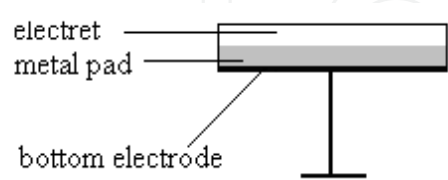
Fig. 3. Schematic diagram of the electret storage in the vacuum chamber in the absence of a second electrode.
