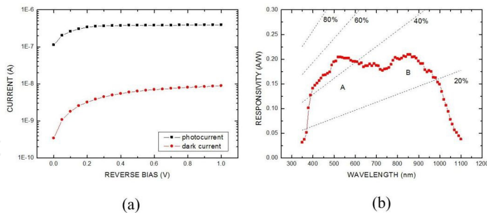
Figure 2. a) The dark and illuminated ( \lambda=530 nm) I-V characteristics of the p -ZnO/ n -Si heterostructure photodiode. (b) The responsivity as a function of the wavelength for a p -ZnO/ n -Si heterostructure photodiode at a bias of 1 V [25].
