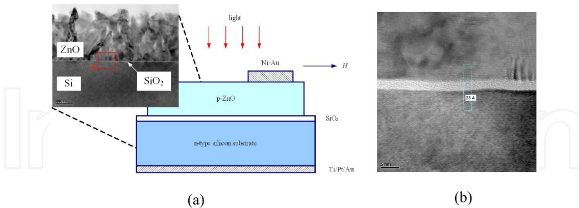
Figure 6. a) Schematic cross-section of the complete structure. (b) Cross sectional TEM image of p\text{-ZnO}/\text{SiO}_2 ultrathin interlayer/ n\text{-Si} structure [49,51].
