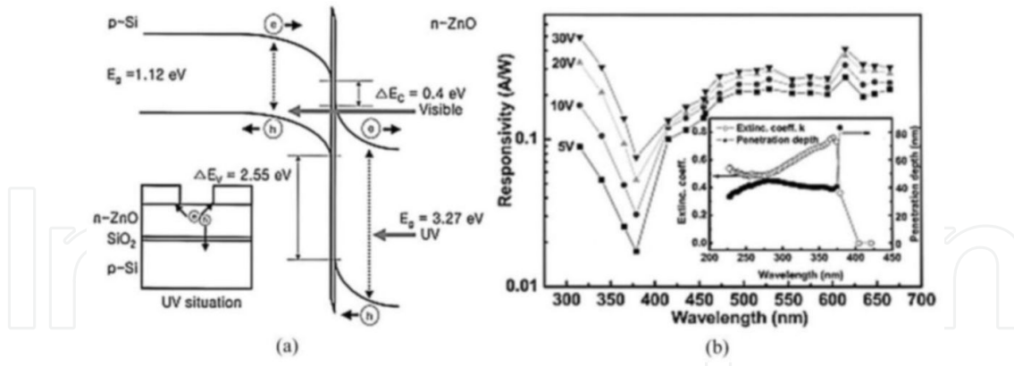
Figure 5. a) Energy-band diagram of a reverse-biased n-ZnO/p-Si structure. (b) Spectral responsivity curves obtained under the reverse biases [52].
