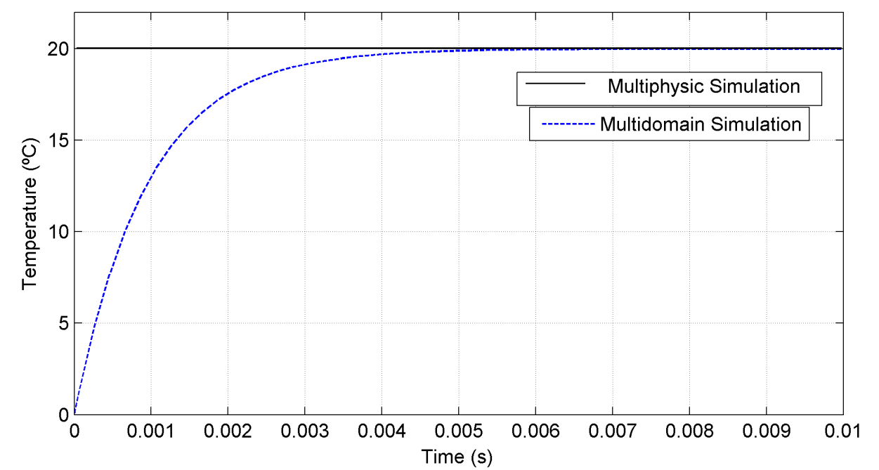
Fig. 16. Stabilization time to room temperature.
