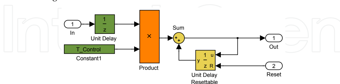
Fig. 5. Substitute for the Forward-Euler Discrete Integrator block with external reset.
