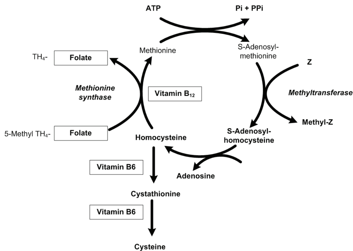
Fig. 2. Homocysteine metabolism
