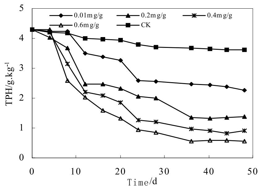
Fig. 15. Residual TPH concentration in soil as a function of bacteria dosage and time.
