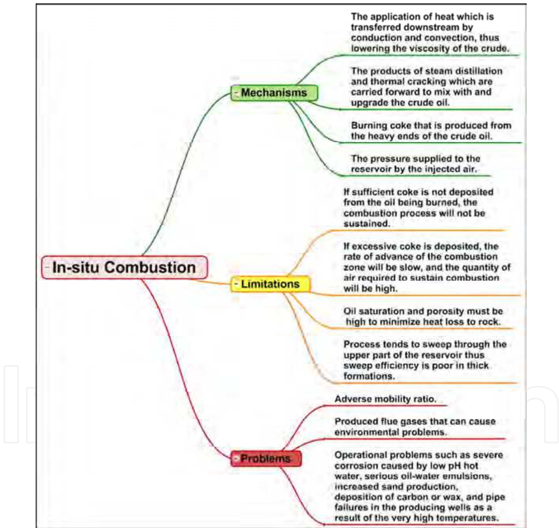
Fig. 16. In-situ Combustion: mechanisms, limitations, and problems (Adapted from Lyons & Plisga, 2005).
