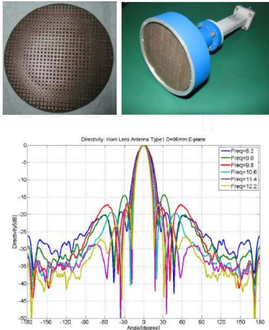
Fig. 23. (a) The 3D flat-lens antenna made of gradient index metamaterial. The aperture size is 9.6 cm. (b) The measured far-field radiation patterns of the 3D metamaterial flat lens antenna in the X band.
