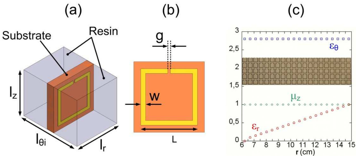
Fig. 6. (a) Unit cell. (b) The dimensions of a typical square SRR are: L=3.6 mm, w=0.3 mm and copper thickness t=35\text{ }\mu\text{m} . The SRRs gap g and l_{\theta i} are the only varying parameters. l_{\theta i} linearly decreases from the outer to the inner boundary of the cloak.
