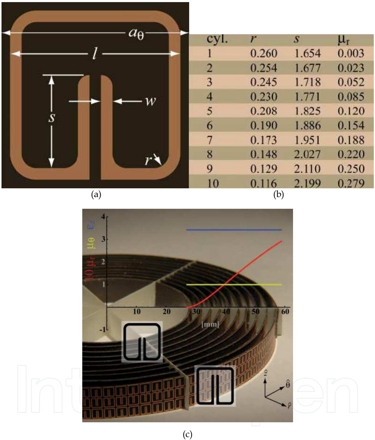
Fig. 3. (a) Elementary cell of the metamaterial. (b) values of the parameters. (c) Photography of the prototype. The insert shows the variations of \mu_r , \mu_\theta and \epsilon_z .
