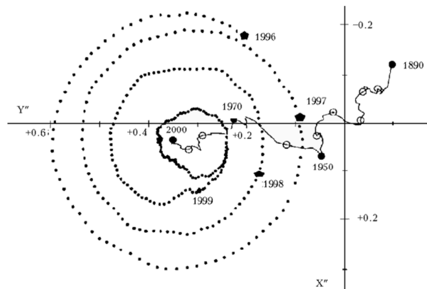
Fig. 5. Wandering of the Earth's North Pole
