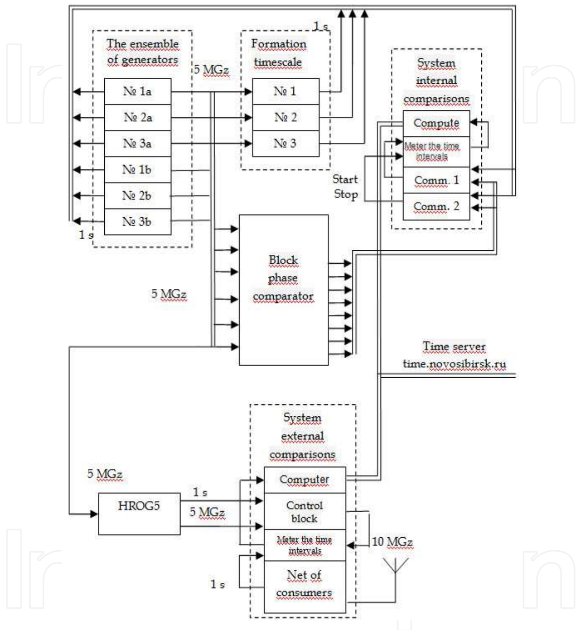
Fig. 1. Block scheme of exact time scale formation equipment
