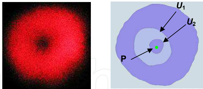
Fig. 16. The partially coherent combined beam (left) and its vector skeleton formed by P and U singularities (right) for completely incoherent mixing of circularly polarized components.
