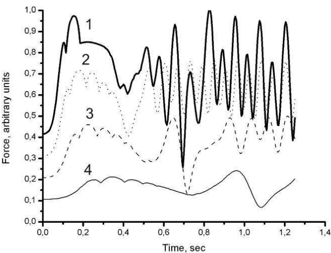
Fig. 8. The change of the resultant force of the test particle motion in the time-averaged field of distributed Poynting vectors with the change of the degree of mutual coherence of the waves (four superposing waves are in phase): curve 1 – one of the waves is incoherent with all other waves; curves 2, 3 and 4 correspond to the degree of coherence of the waves 0.25, 0.5, and 0.75, respectively.
