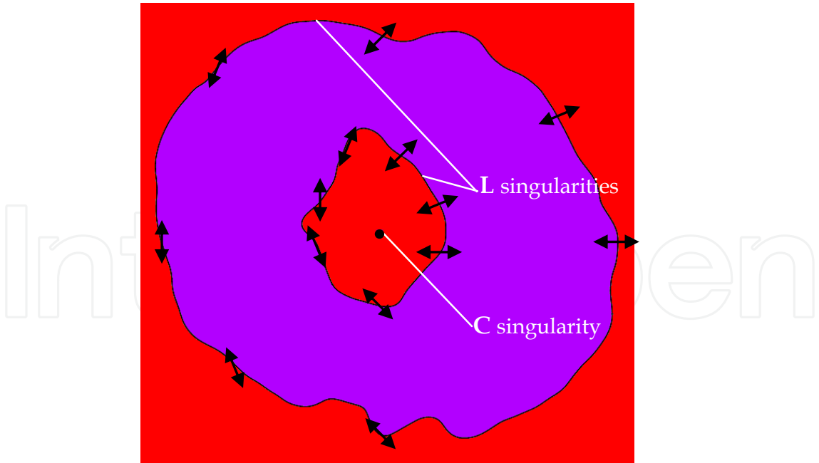
Fig. 18. C and L singularities in combined beam assembled from completely mutual coherent orthogonally (circularly) polarized LG01 mode and plane wave. At L lines, where intensities of two mixed component are equal, the azimuth of polarization changes in agreement of prediction illustrated in Fig. 14 Areas of different colors correspond to opposite handedness.
