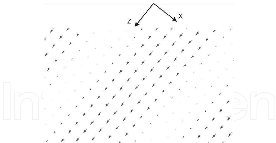
Fig. 2b. Spatial distribution of the time-averaged Poynting vectors resulting from superposition of two orthogonally linearly polarized waves with an interference angle of 90^\circ .
