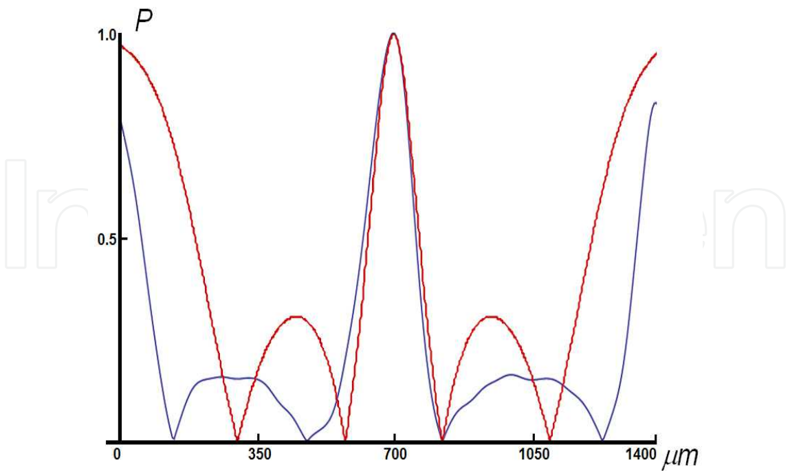
Fig. 17. 1D distribution of the degree of polarization of the combined beam formed by two mutually incoherent orthogonally polarized components defined in Fig.12 and shown in Fig. 16.
