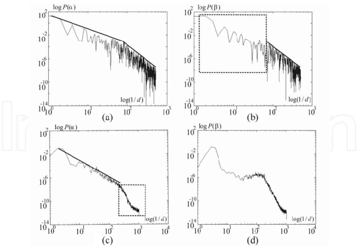
Fig. 25. log-log dependences of power spectra of the azimuth of polarization and ellipticity at images of physiologically normal (a), (b) and pathologically changed (c), (d) skin derma.
