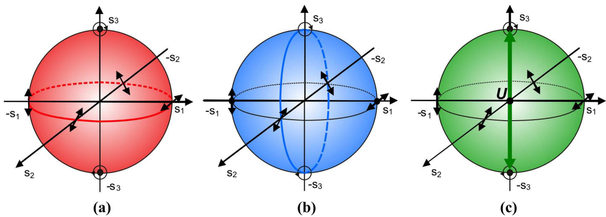
Fig. 13. The lines of equal intensities of orthogonally polarized beams at Stokes space: equator of the Poincare sphere for circular polarization basis, coherent mixing (a); 45°-meridian including the poles for linear polarization basis, coherent mixing (b); diameter of the Poincare sphere connecting the poles for circular polarization basis, incoherent mixing (c).
