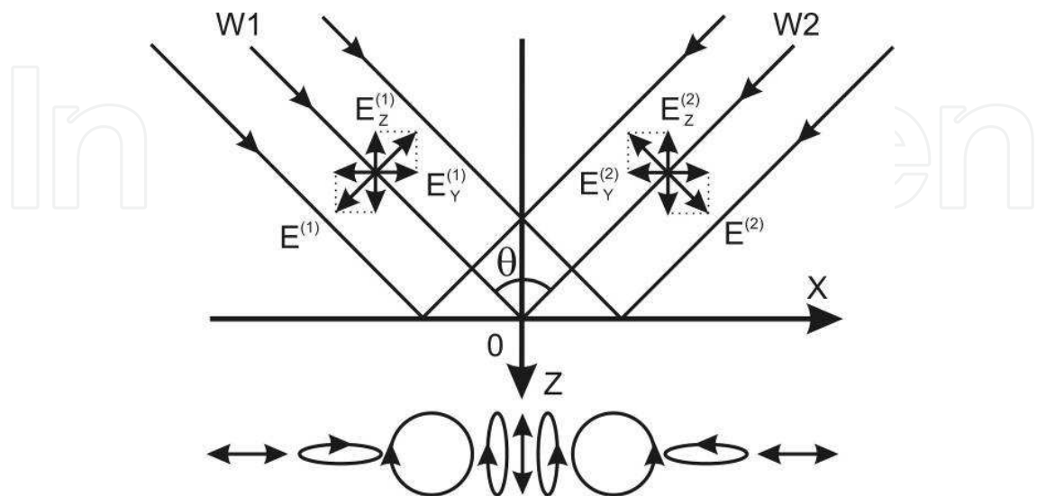
Fig. 2a. Superposition of plane waves of equal amplitudes linearly polarized in the plane of incidence having an interference angle of 90^\circ . Periodical spatial polarization modulation takes place in the plane of incidence.
