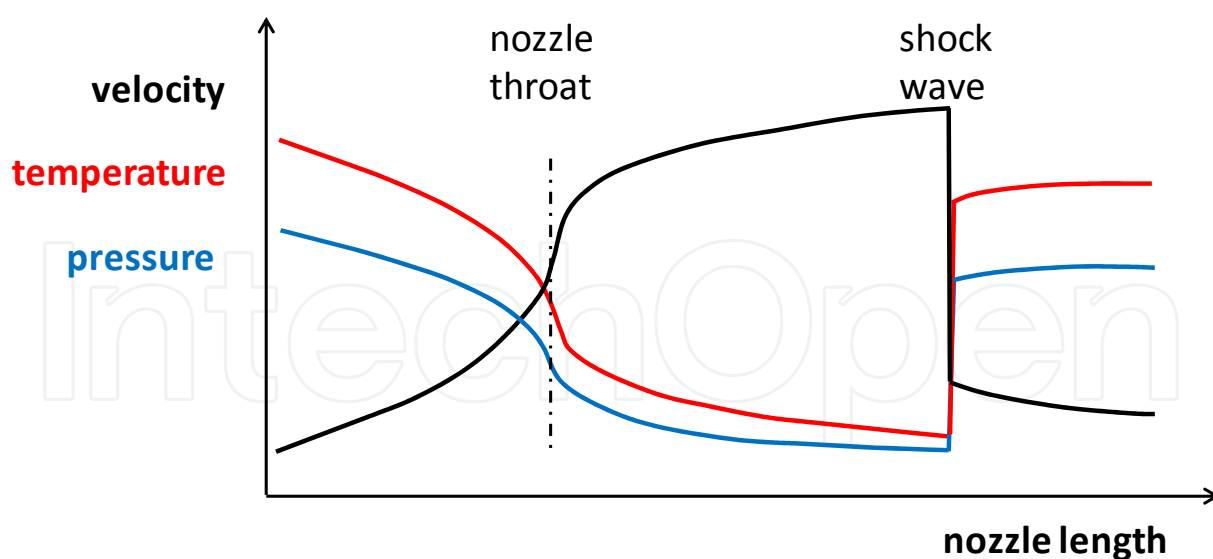
Figure 9. Profile of pressure, temperature and velocity of a gas passing through the supersonic nozzle
