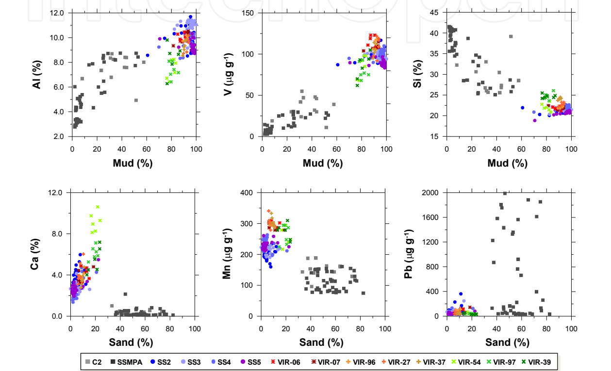
Fig. 2. Scatterplots of element concentrations vs mud (<63 µm) or sand contents in core samples (N = 210) from different sectors of the Ría de Vigo (core depths between 0.24 and 3.10 m): inner ría both intertidal (squares) and subtidal (circles) sediments, middle ría (doble crosses), middle-outer ría (crosses) and outer ría (vanes). Metal concentrations obtained from X-ray fluorescence (XRF) analyses. Note the positive correlation between Al or V vs mud and Ca vs sand, and the negative correlation between Si vs mud and Mn vs sand contents. Note also the extremely high values of Pb in the intertidal sediments. Sample location in Fig. 1.
