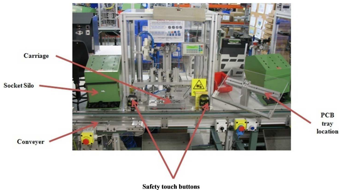
Fig. 5. Assembly jig for single gang switches
