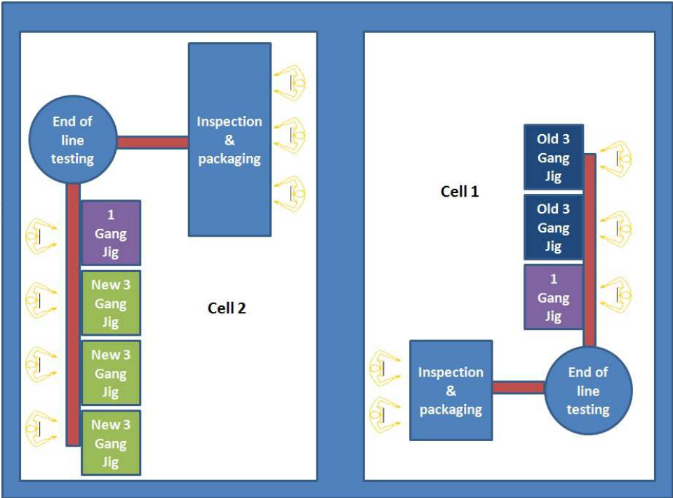
Fig. 11. Proposed layouts for Cell 1 and Cell 2 (Concept 2)
