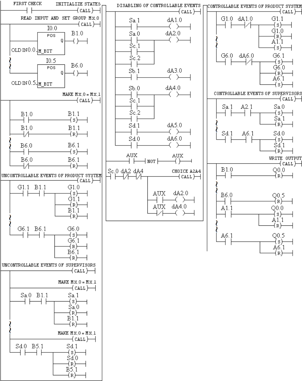
Fig. 12. PLC implementation for the case study
