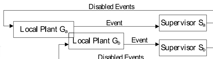
Fig. 2. Local modular supervisory control architecture (Queiroz & Cury, 2002)
