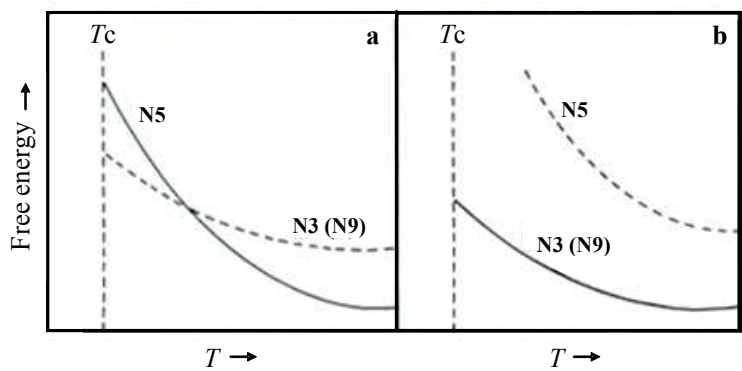
Fig. 6. Schematic figures of temperature dependence of free energy change of N5- and N3- or N9- type NaYPSi in the cases assuming N5- (a) and N3- (b) or N9-type (b) NaYPSi as the high temperature-stable phase, where T_c is the crystallization temperature.
