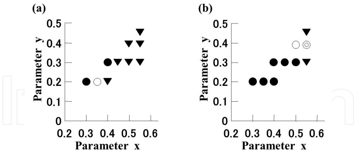
Fig. 15. The diagrams of phase-composition of NYGeS glass-ceramics heated at 900°C (a) and 1000°C (b) for 5 h. ● Na 5 RSi 4 O 12 (N5) ▼ Na 9 RSi 6 O 18 (N9) ○ N5+N3 ⊙ N5+N9
