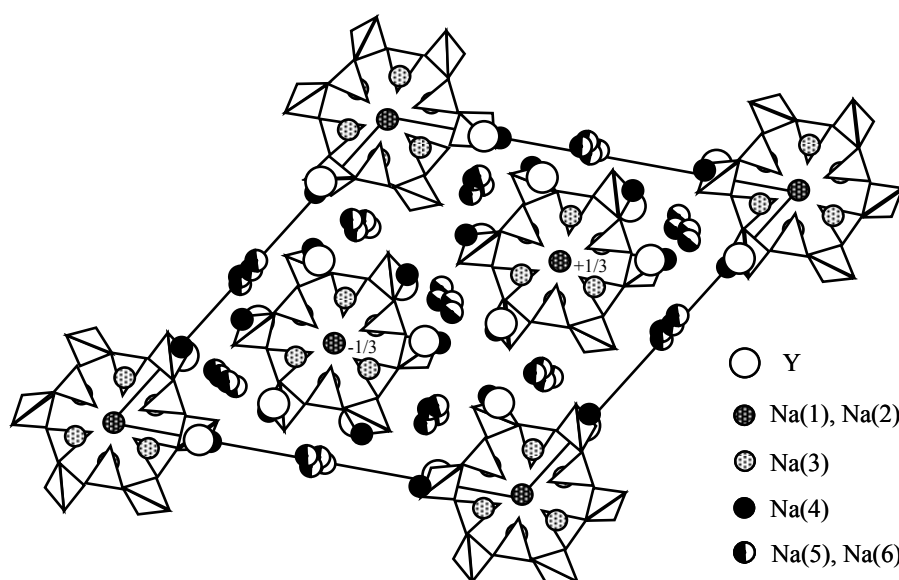
Fig. 1. Crystal Structure of \text{Na}_5\text{YSi}_4\text{O}_{12} . Projection of the \text{Na}_5\text{YSi}_4\text{O}_{12} Structure on (100).
