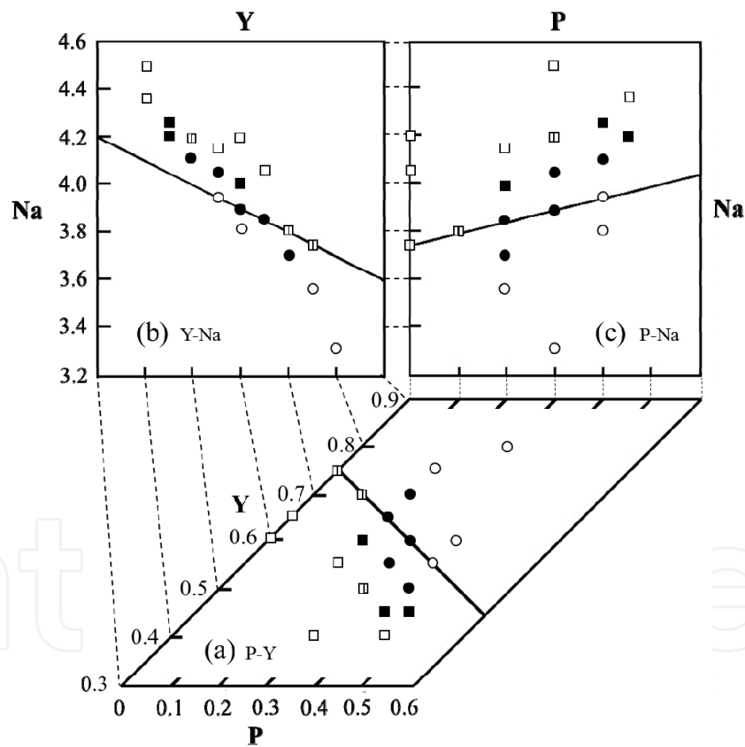
Fig. 4. Composition dependence of precursor ( pp ) and high temperature-stable phases ( sp ) of glass-ceramic NaRPSi on P-Y (a), Y-Na (b) and P-Na (c) maps, where precursor phases N3 and N9 are shown with circles and squares , respectively. High temperature-stable phases are shown in such a way that solid marks means that N5-NaRSi is the stable, while open marks indicate that the precursor phases are also stable even at high temperatures. Mixed phases are also shown: open circle pp = sp = N3 ; filled circle pp = N3 , sp = N5 ; open square pp = sp = N9 ; filled circle pp = N9 , sp = N5 ; open split square pp = N9 , sp = N9 + N5
