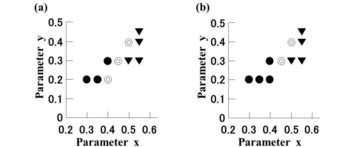
Fig. 16. The diagrams of phase-composition of NYTeS glass-ceramics heated at 900°C (a) and 1000°C (b) for 5 h. ● Na 5 RSi 4 O 12 (N5) ▼ Na 9 RSi 6 O 18 (N9) ⊙ N5+N9
