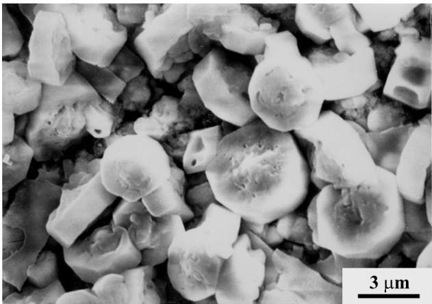
Fig. 13. SEM photograph of the specimen with Na 3.9 Sm 0.6 P 0.3 Si 2.7 O 9 composition heated at 900°C by the pattern (C).
