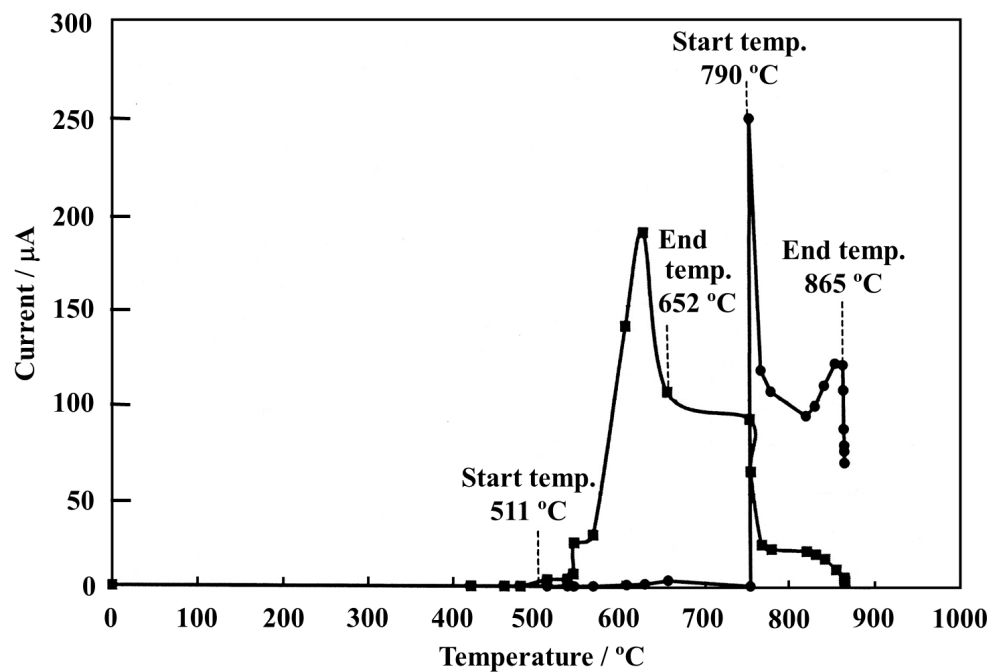
Fig. 19. Current profile in relation to temperature measured by applying voltage in two limited temperature ranges.
