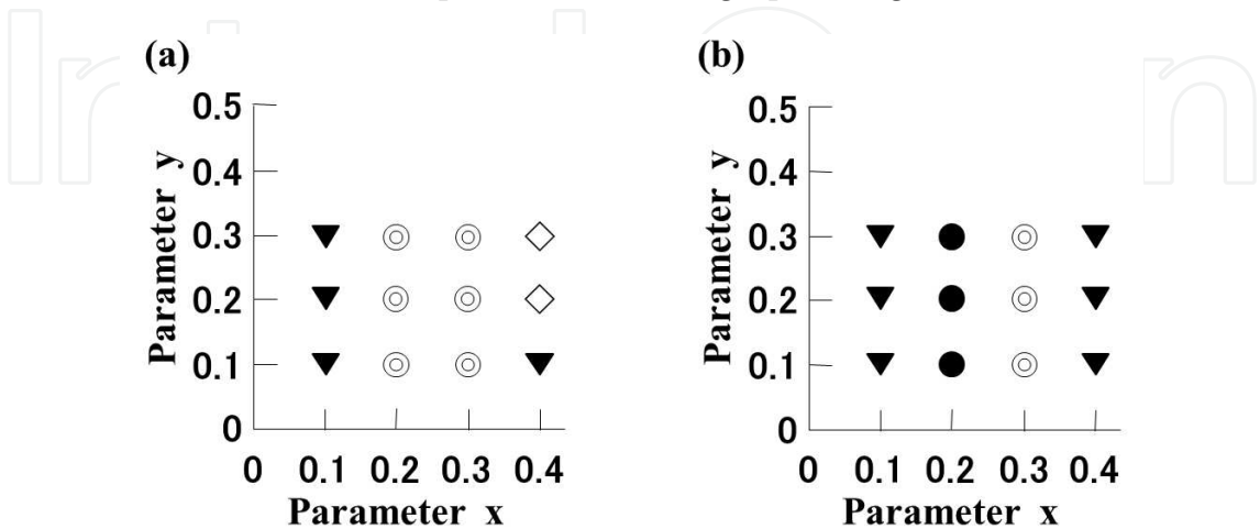
Fig. 14. The diagrams of phase-composition of NYTiS glass-ceramics heated at 900°C (a) and 1000°C (b) for 5 h. ● Na 5 RSi 4 O 12 (N5) ▼ Na 9 RSi 6 O 18 (N9) ○ N5+N9 ◇ N3+N9
