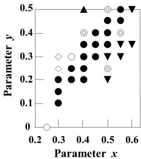
Fig. 12. The diagram of phase-composition of NaSmPSi glass-ceramics crystallized at 900°C. ●Na 5 YSi 4 O 12 (N5) type, ▲Na 3 YSi 3 O 9 (N3) type, ▼Na 9 RSi 6 O 18 (N9) type ○N5+N3, ⊙N5+N9, ◇N3+N9
