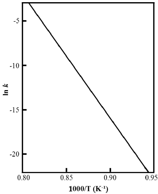
Fig. 9. Arrhenius-type plot of ln k with 1000/ T of specimen Na 3.9 Y 0.6 Si 2.7 O 9 .
