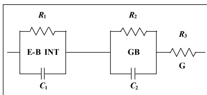
Fig. 2. Equivalent circuit employed for the admittance analysis.
