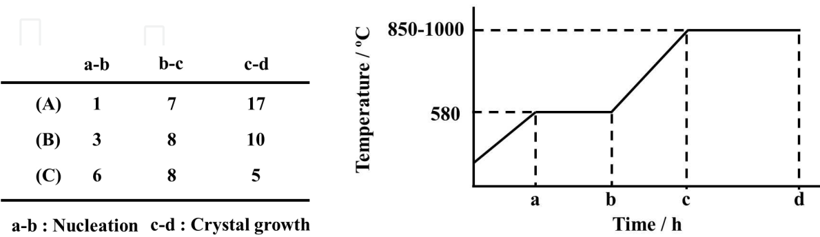
Fig. 11. Program of temperature and time for the production of NaSmPSi glass-ceramics. Samples were prepared according to the chemical formula mentioned above of Na 3+3x-y Sm 1-x P y Si 3-y O 9 . The temperatures employed for nucleation and crystallization of glass specimens were also determined by the results of DTA analysis. Fig. 11 shows the program of temperature and time for the production of glass-ceramic NaSmPSi employed in the present work. The N5-type NaSmPSi ionic conductors were successfully produced by crystallization of glasses. Although the glass samples heated by the program pattern (A) shown in Fig. 11 broke during crystallization and the glass-ceramic NaSmPSi obtained by the pattern (B) was difficult to prevent from cracking during crystallization, most of the NaSmPSi compounds by the pattern (C) were obtained as crack free bulky glass-ceramics (the glass samples broke during crystallization when heating time for crystallization was over 5 h). Fig. 12 shows the phase-composition diagram of samples crystallized at 900°C by the pattern (C). The crystallization of the N5 single-phase glass-ceramic NaSmPSi was dependent strongly on the concentrations of both [R] and [P] (or x and y in the composition parameters) and the temperature for crystallization of glass specimens. Fig. 13 shows SEM photograph of microstructure of specimen with the Na 3.9 Sm 0.6 P 0.3 Si 2.7 O 9 composition heated at 900°C by the pattern (C). The grain size of the specimen was about 3-5 μm. The state of grain growth is promoted with increase of heating temperature and heating time for crystallization. Although grain growth may cause high conductivity, it was difficult to prevent the sample heated for a long time from cracking during crystallization. Studies are underway to produce a crack free sample. Conduction properties were measured by the ac two-probe method on cylindrical glass-ceramics of typically 15 mm in diameter and 2 mm in thickness with an LF impedance analyzer. Electrodes were prepared by sputtering of gold on polished surfaces. The applied ac field ranged from 5 to 10 MHz in frequency. The temperature dependence of the conductivity was measured in a similar way at several temperatures ranging from room temperature to 350°C. Table 3 summarizes the conduction properties of the N5-type glass-ceramic NaSmPSi specimens. It was found that NaSmPSi containing the largest Sm 3+ ions was less conductive than NaYPSi with medium Y 3+ ions as the grain sizes of the presented specimens were very small.
