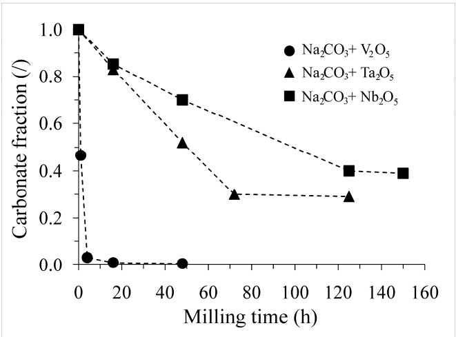
Fig. 14. Fraction of carbonate, determined by TG analysis, as a function of milling time in Na 2 CO 3 -M 2 O 5 (M = V, Nb, Ta) powder mixtures. The lines are drawn as a guide for the eye (from Rojac et al., 2011).
