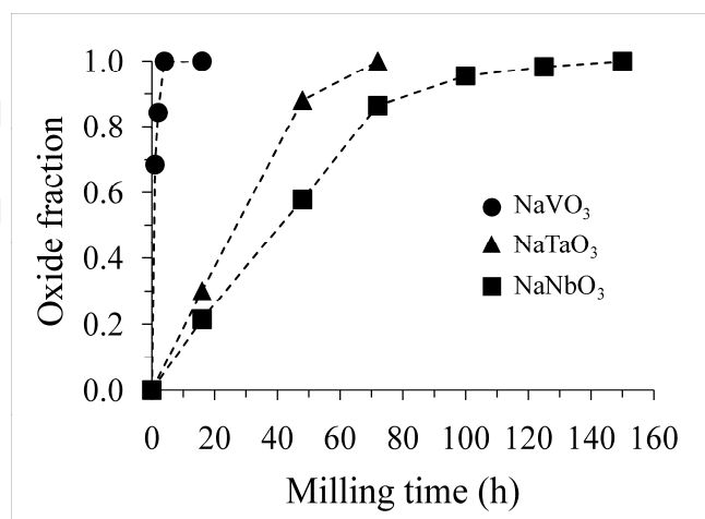
Fig. 11. Fraction of \text{NaMO}_3 ( \text{M} = \text{V}, \text{Nb}, \text{Ta} ), determined by Rietveld refinement analysis, as a function of milling time. The lines are drawn as a guide for the eye (from Rojac et al., 2011).
