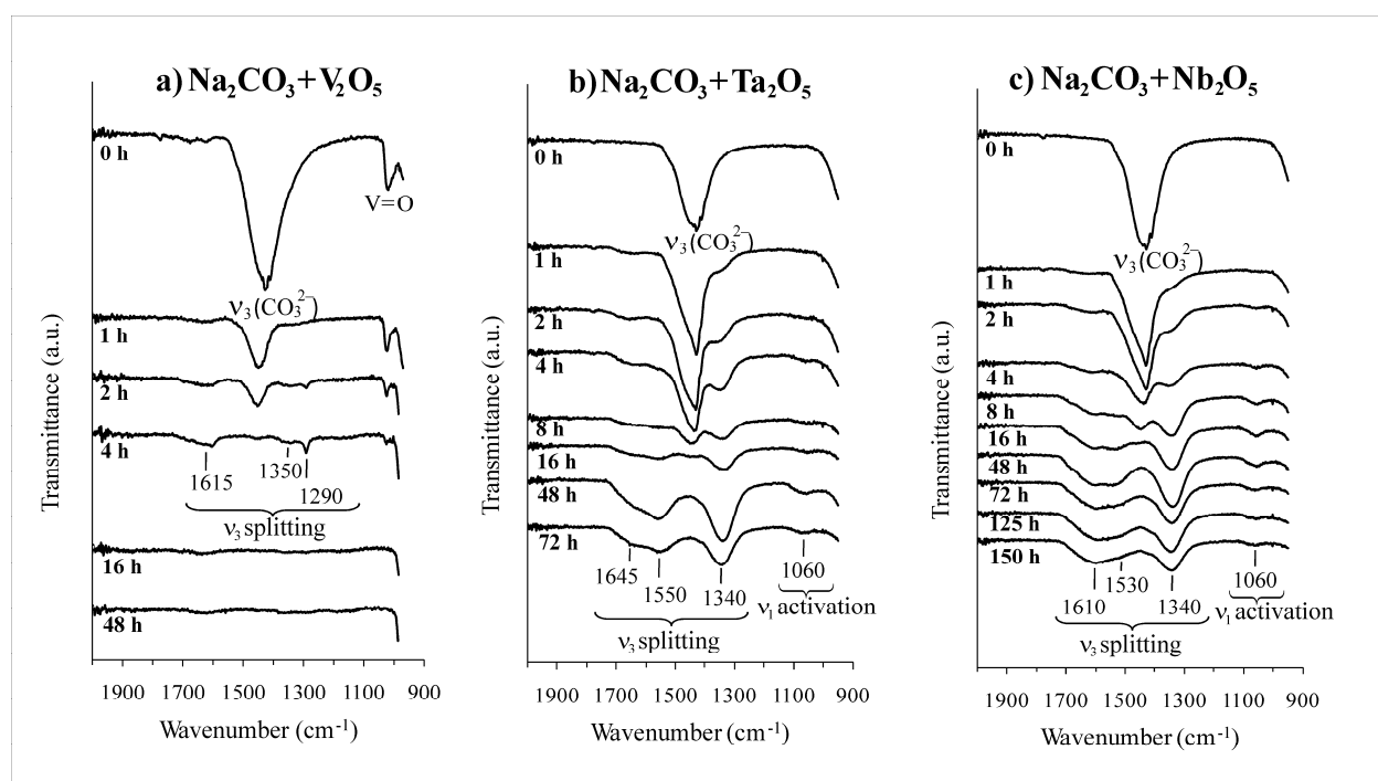
Fig. 12. FT-IR spectra of \text{Na}_2\text{CO}_3\text{--M}_2\text{O}_5 ( M = \text{V}, \text{Nb}, \text{Ta} ) powder mixtures after different milling times (from Rojac et al., 2011).
