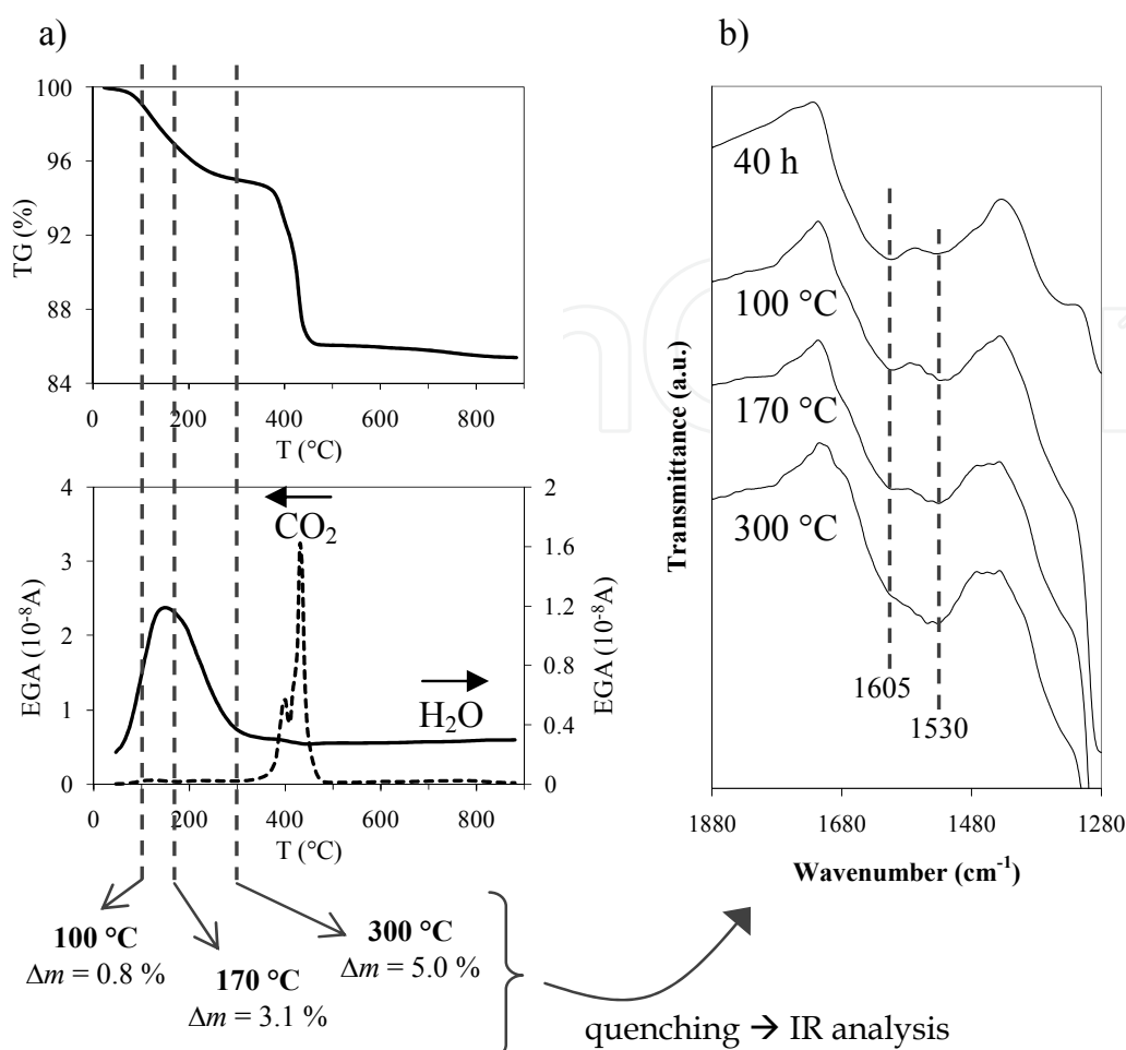
Fig. 10. a) TG and EGA( \text{H}_2\text{O} , \text{CO}_2 ) curves of the 40-hours high-energy milled \text{Na}_2\text{CO}_3 - \text{Nb}_2\text{O}_5 powder mixture. The dashed lines on the graphs represent the temperatures at which the 40-hours milled sample was air-quenched. b) FT-IR spectra of the 40-hours high-energy milled \text{Na}_2\text{CO}_3 - \text{Nb}_2\text{O}_5 powder mixture air-quenched from various temperatures (from Rojac et al., 2006).
