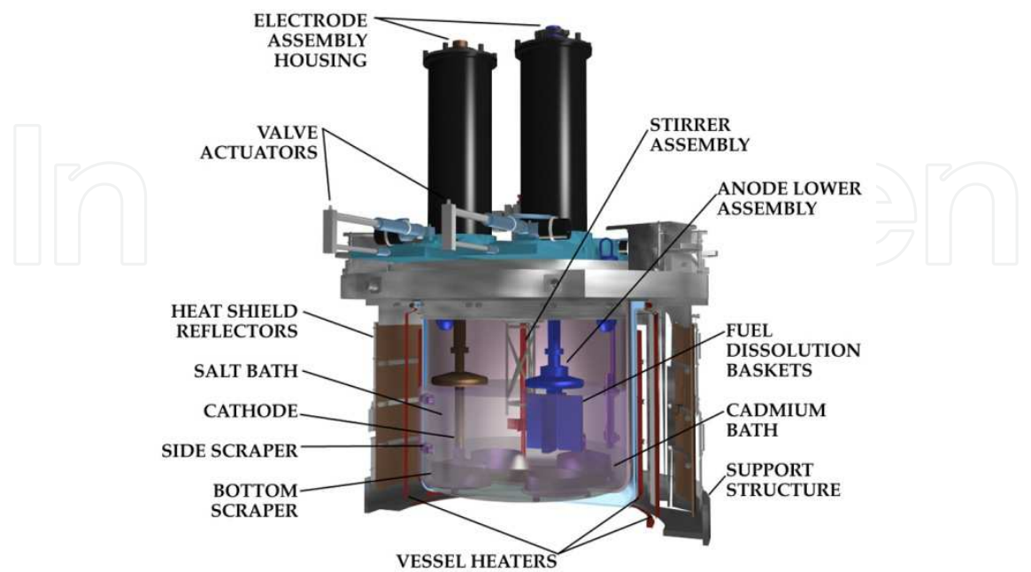
Fig. 3. Electrorefiner.
