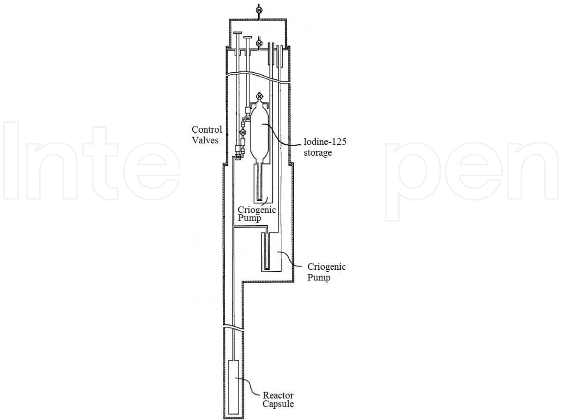
Fig. 1. Iodine-125 production system in cryogenic method [Zeituni et. Al., 2011]. (To publisher, this is too small. To authors, please indicate how to use this unit showing or describing the corresponding reactor part or position: for exapmle, “The reactor capsule part is placed into the reactor core.” The figure is not enough to explain how to retrieve the capsule, where to insert next capsule, where to take up the I-125.)
