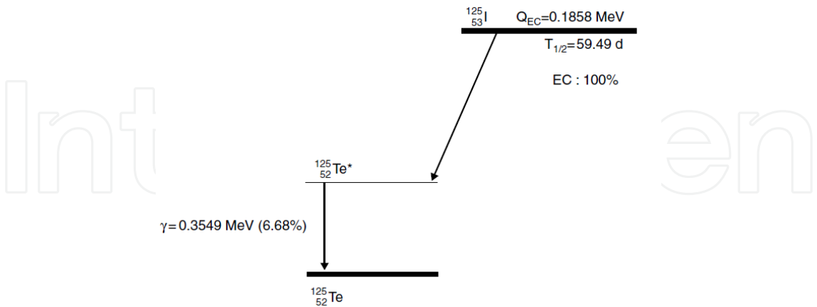
Fig. 2. Iodine-125 decay scheme [Baltas et. Al, 2006]
