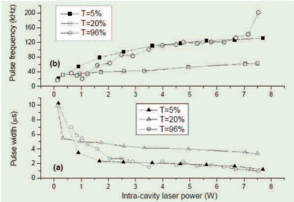
Fig. 25. Output coupling dependence of (a) pulse width and (b) pulse frequency under different intra-cavity power levels.
