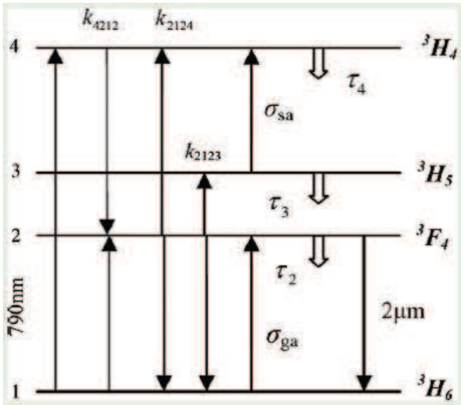
Fig. 26. Schematic of the four lowest energy manifolds in \text{Tm}^{3+} ions.
