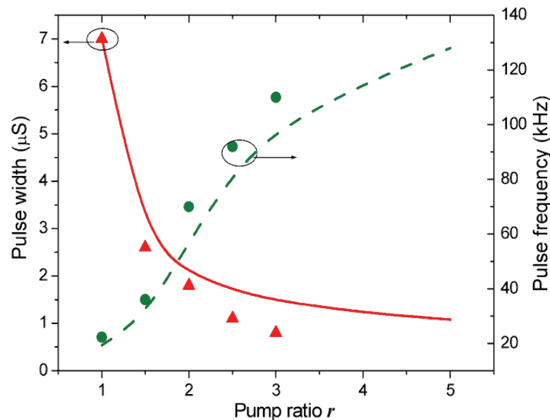
Fig. 36. Pulse width and pulse frequency of the Tm 3+ -doped fiber laser with T~96% output coupler at various pump levels. The solid and dotted lines show the simulation results, and the triangle and circle dots indicate the experimental results.
